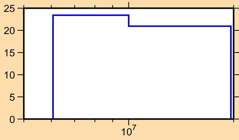
\Delta\sigma/\sigma vs. E for ^{204}\text{Pt}(n,\text{nonel.})
