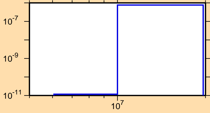
\sigma vs. E for ^{204}\text{Pt}(n,\alpha)
