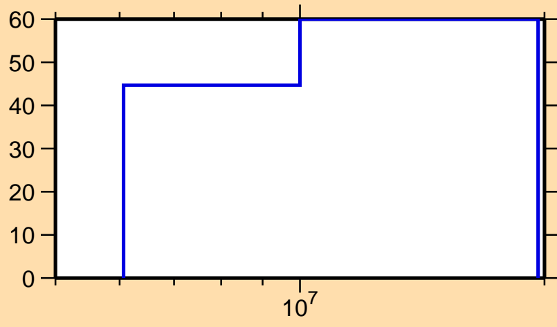
\Delta\sigma/\sigma vs. E for ^{204}\text{Pt}(n,2n)
