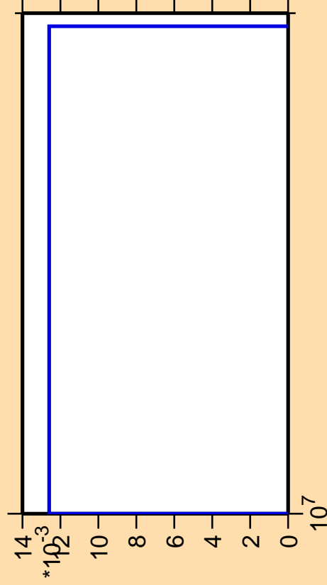
\Delta\sigma/\sigma vs. E for ^{204}\text{Pt}(n,2np)
