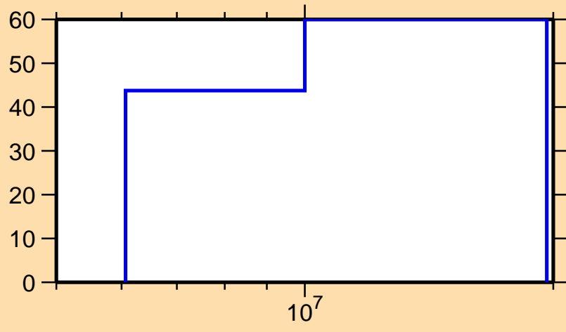
\Delta\sigma/\sigma vs. E for ^{204}\text{Pt}(n,ncont.)
