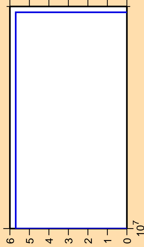
\Delta\sigma/\sigma vs. E for ^{204}\text{Pt}(n,\text{nd})
