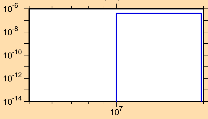
\sigma vs. E for ^{204}\text{Pt}(n,t)
