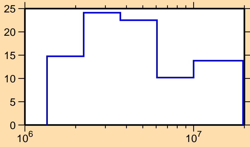
\Delta\sigma/\sigma vs. E for ^{204}\text{Pt}(n, el.)
