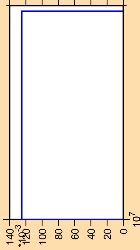
\Delta\sigma/\sigma vs. E for ^{204}\text{Pt}(n,2n\alpha)
