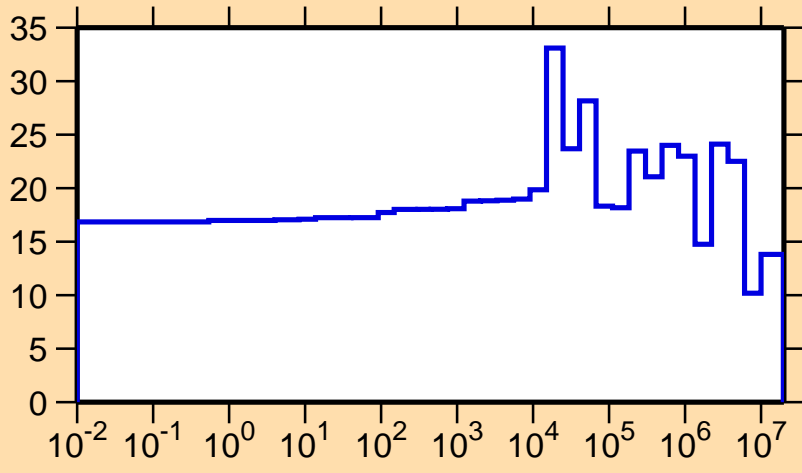
\Delta\sigma/\sigma vs. E for ^{204}\text{Pt}(n,\text{el.})
