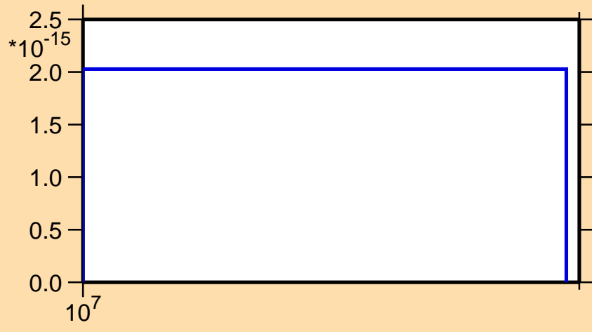
\sigma vs. E for ^{204}\text{Pt}(n,2np)
