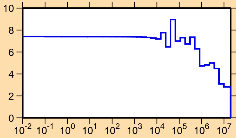
\sigma vs. E for ^{204}\text{Pt}(n,\text{el.})
