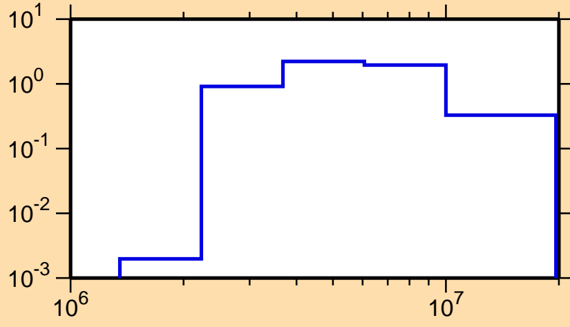
\sigma vs. E for ^{204}\text{Pt}(n,n\text{cont.})
