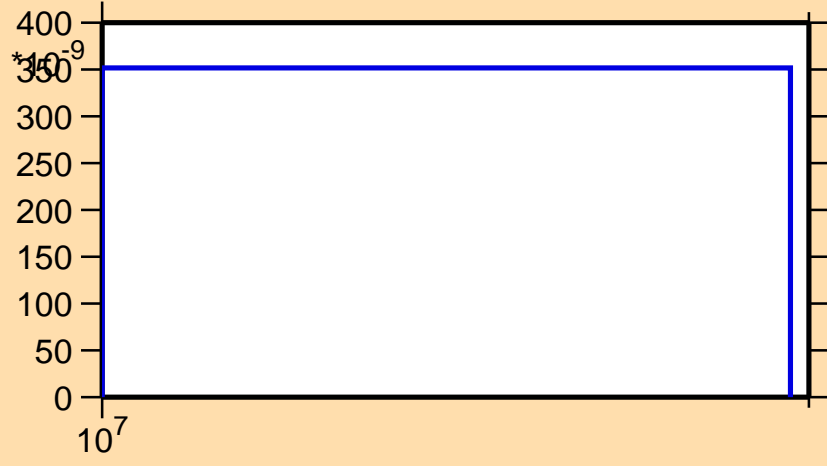
\sigma vs. E for ^{204}\text{Pt}(n,np)
