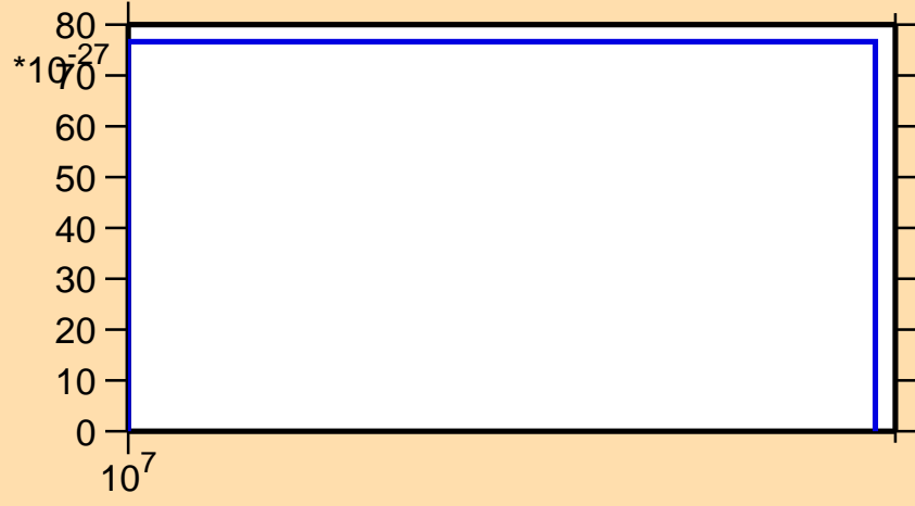
\sigma vs. E for ^{204}\text{Pt}(\text{mt } 11)
