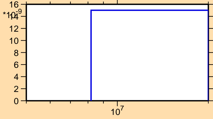
\sigma vs. E for ^{204}\text{Pt}(n,n\alpha)
