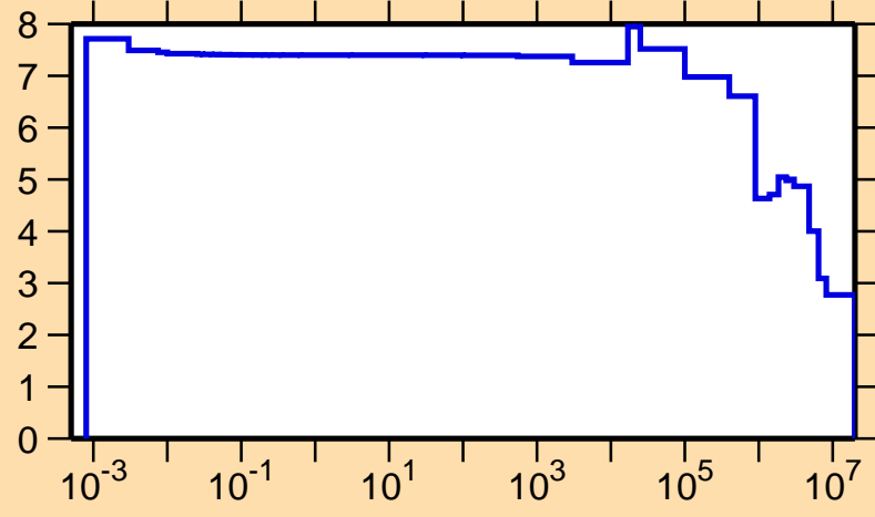
\sigma vs. E for ^{204}\text{Pt}(n,\text{el.})
