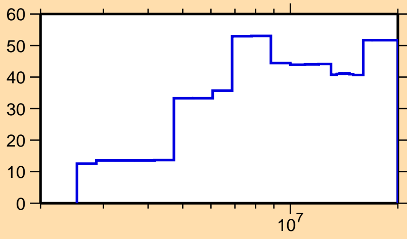
\Delta\sigma/\sigma vs. E for ^{205}\text{Pt}(n,n\text{cont.})
