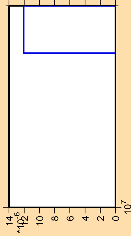
\Delta\sigma/\sigma vs. E for ^{206}\text{Pt}(\text{mt } 42)
