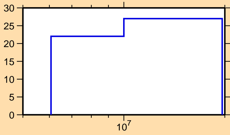
\Delta\sigma/\sigma vs. E for ^{206}\text{Pt}(n,ncont.)
