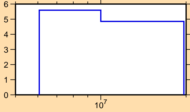
\Delta\sigma/\sigma vs. E for ^{206}\text{Pt}(n, \text{tot.})
