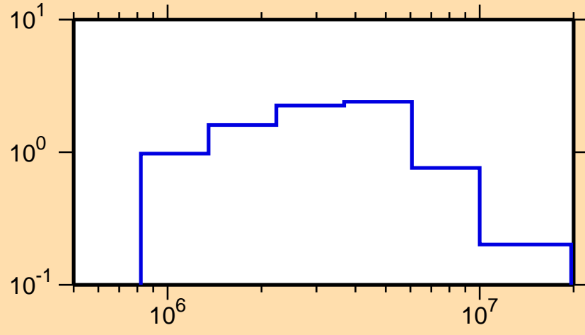
\sigma vs. E for ^{206}\text{Pt}(n,\text{inel.})
