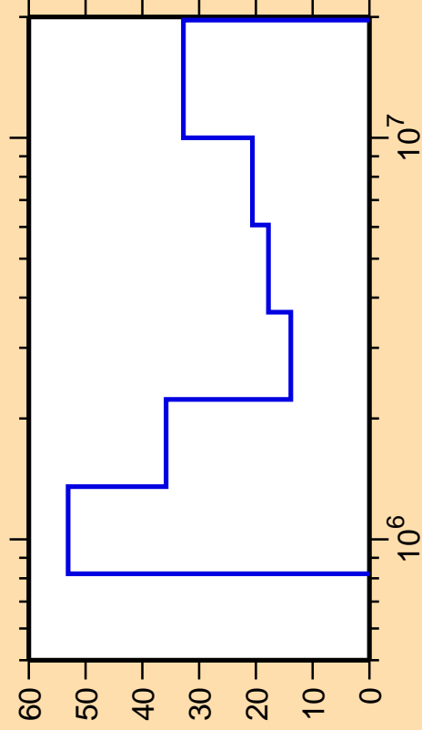
\Delta\sigma/\sigma vs. E for ^{206}\text{Pt}(n,\text{inel.})
