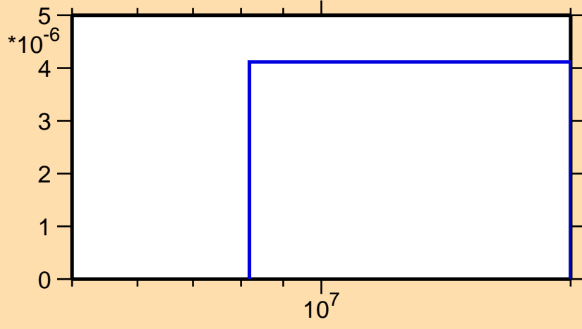
\sigma vs. E for ^{206}\text{Pt}(n,p)
