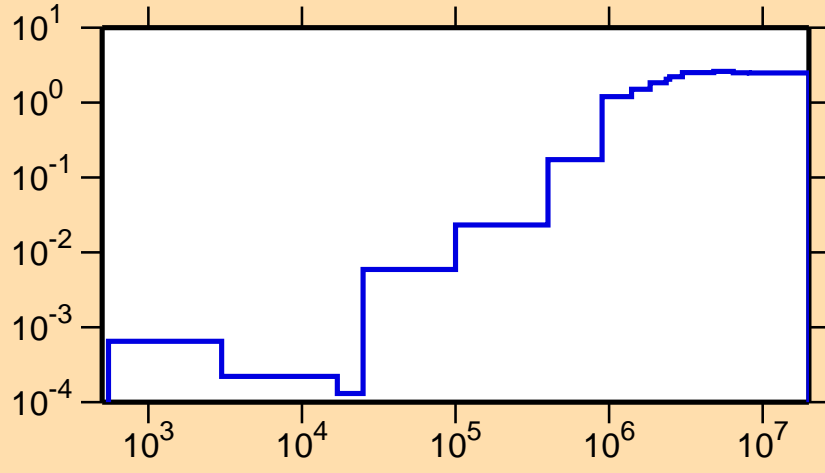
\sigma vs. E for ^{206}\text{Pt}(n,\text{nonel.})
