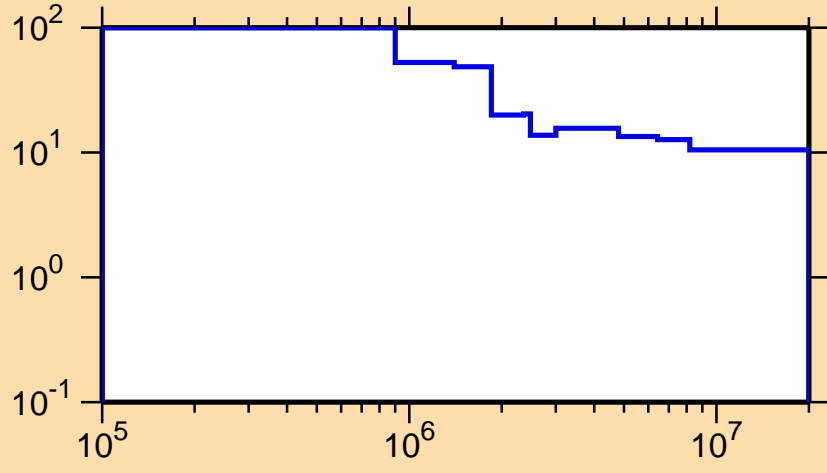
\Delta\sigma/\sigma vs. E for ^{206}\text{Pt}(n, nonel.)
