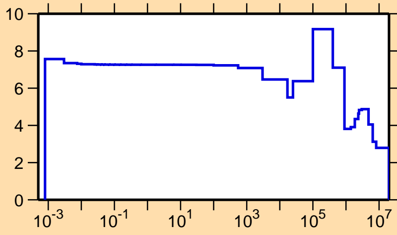
\sigma vs. E for ^{206}\text{Pt}(n,\text{el.})
