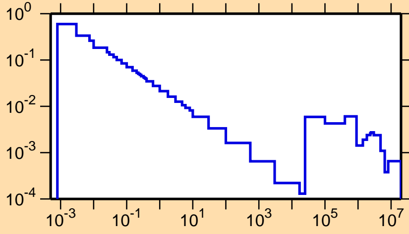
\sigma vs. E for ^{206}\text{Pt}(n,\gamma)
