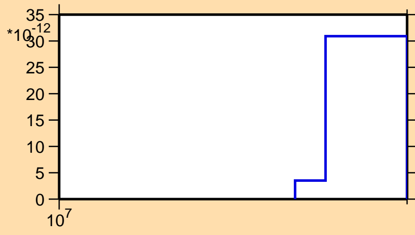
\sigma vs. E for ^{228}\text{Pu}(n,\text{pd})
