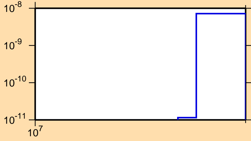
\sigma vs. E for ^{228}\text{Pu}(n,3n\alpha)
