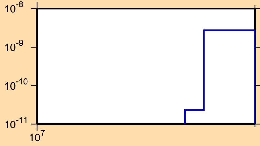
\sigma vs. E for ^{228}\text{Pu}(n,nt)
