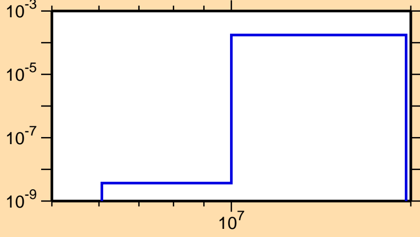
\sigma vs. E for ^{228}\text{Pu}(n,np)
