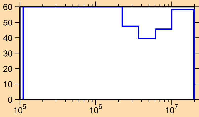
\Delta\sigma/\sigma vs. E for ^{228}\text{Pu}(n, n\text{cont.})
