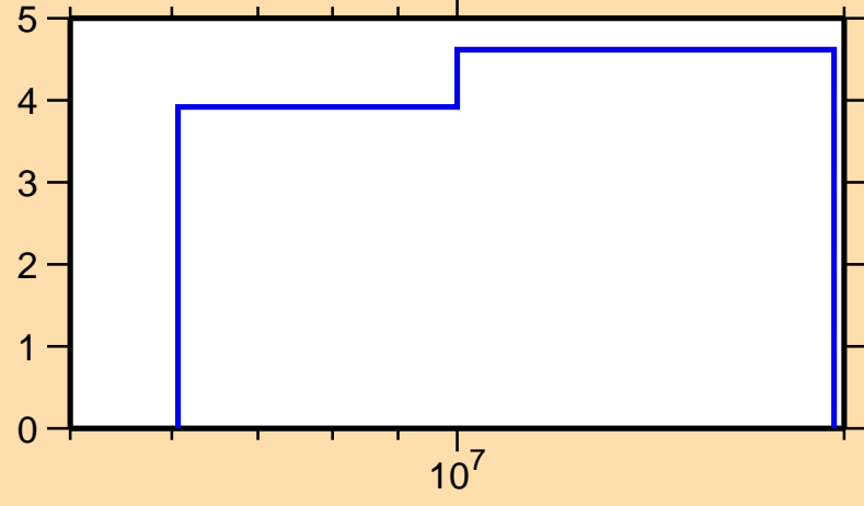
\Delta\sigma/\sigma vs. E for ^{228}\text{Pu}(n,\text{nonel.})
