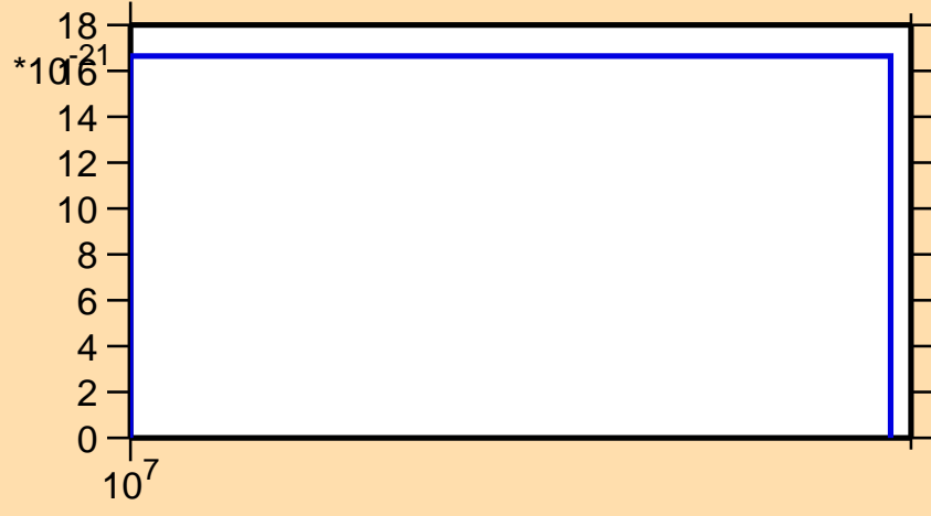
\sigma vs. E for ^{228}\text{Pu} (mt 42)
