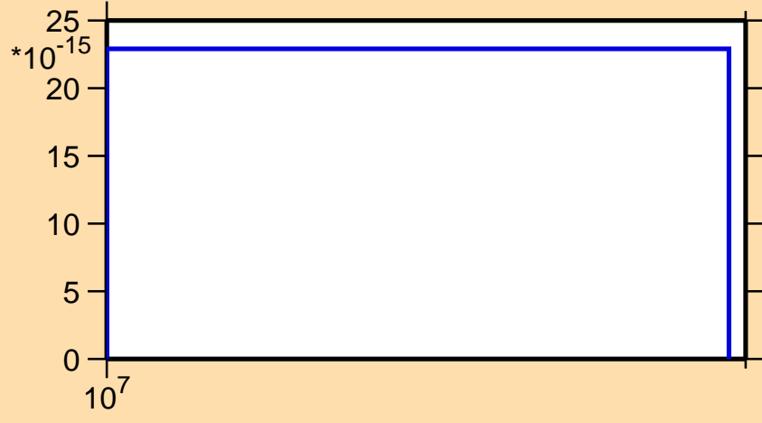
\sigma vs. E for ^{228}\text{Pu} (mt 34)
