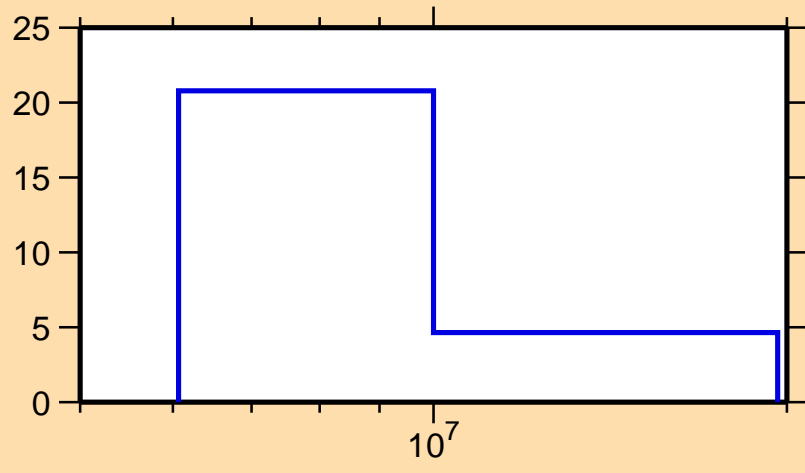
\Delta\sigma/\sigma vs. E for ^{228}\text{Pu}(n,\text{el.})
