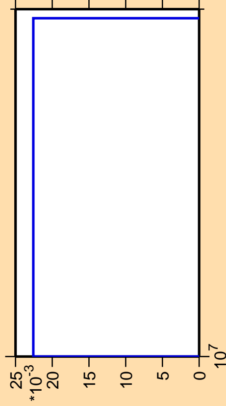
\Delta\sigma/\sigma vs. E for ^{228}\text{Pu} (mt 34)
