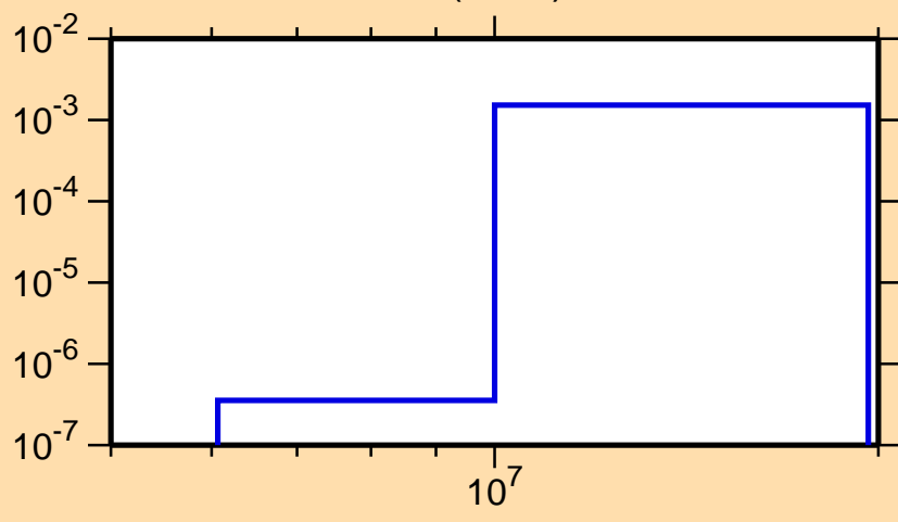
\sigma vs. E for ^{228}\text{Pu}(n,2n)
