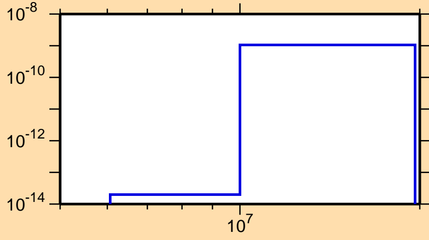
\sigma vs. E for ^{228}\text{Pu}(\text{mt117})
