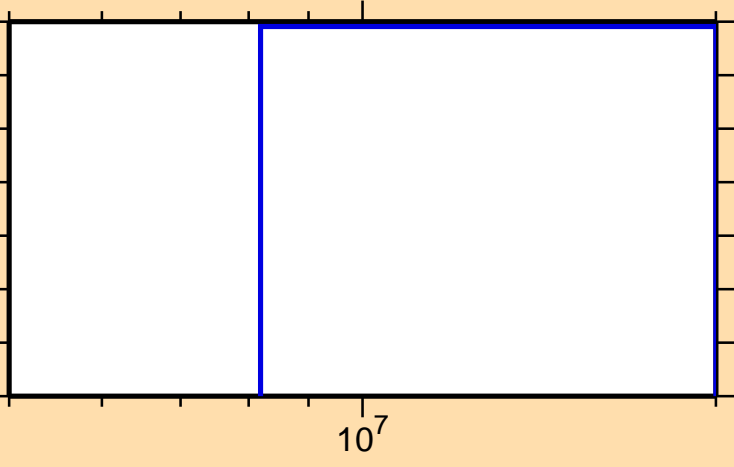
\sigma vs. E for ^{228}\text{Pu}(n,\text{He}3)
