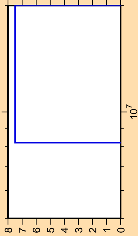
\Delta\sigma/\sigma vs. E for ^{228}\text{Pu}(n,f)
