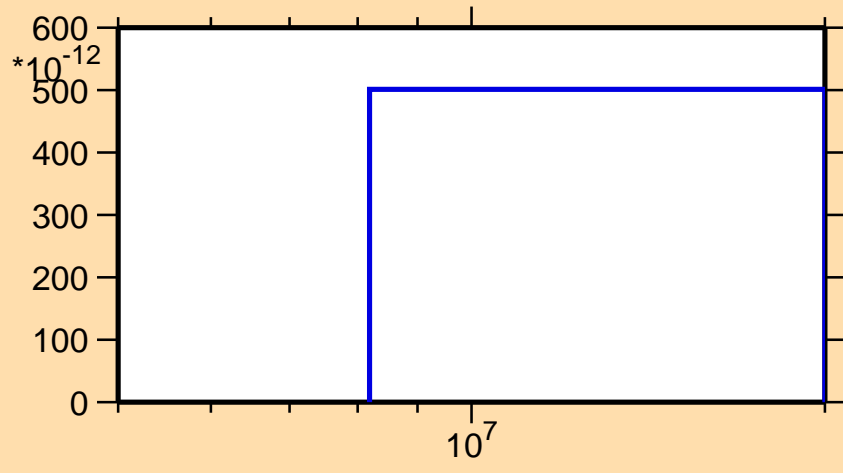
\sigma vs. E for ^{228}\text{Pu}(n,nd)
