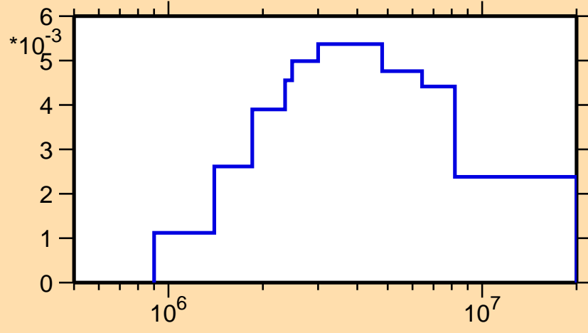
\sigma vs. E for ^{228}\text{Pu}(n,n\alpha)
