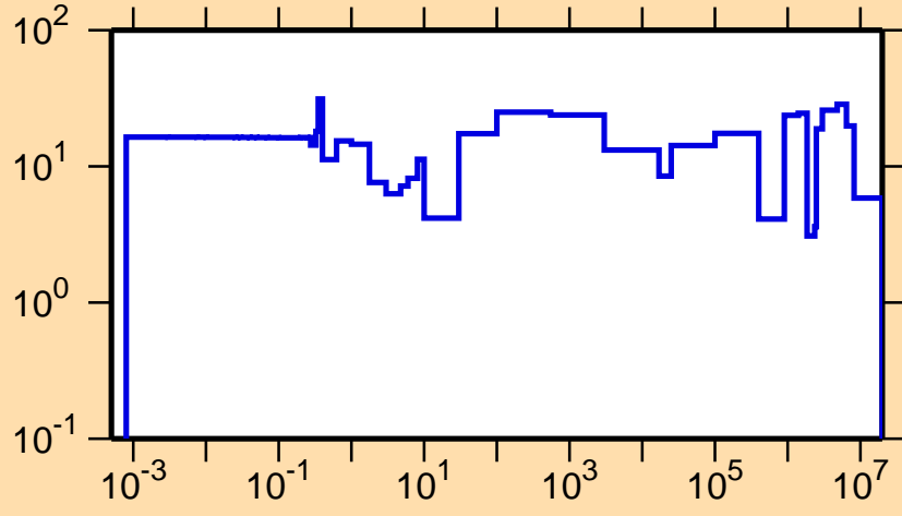
\Delta\sigma/\sigma vs. E for ^{228}\text{Pu}(n,el.)
