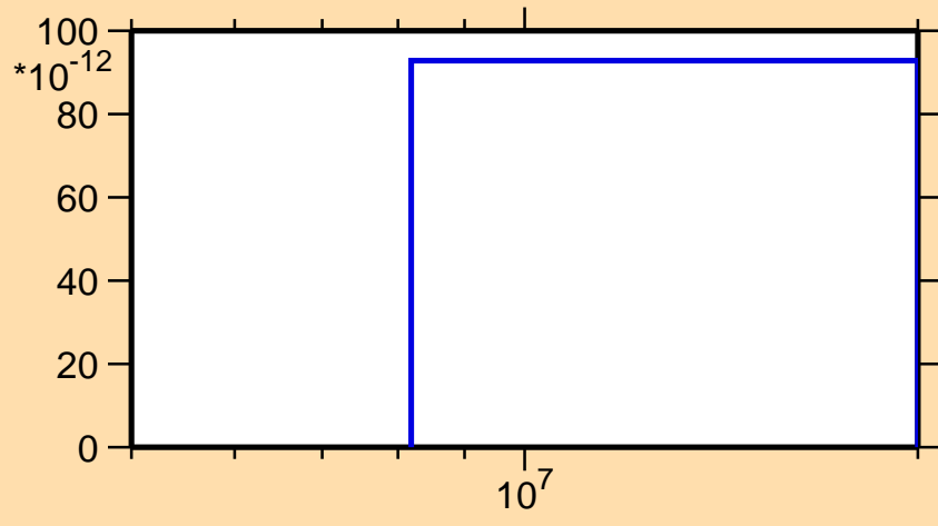
\sigma vs. E for ^{228}\text{Pu}(n,3n)
