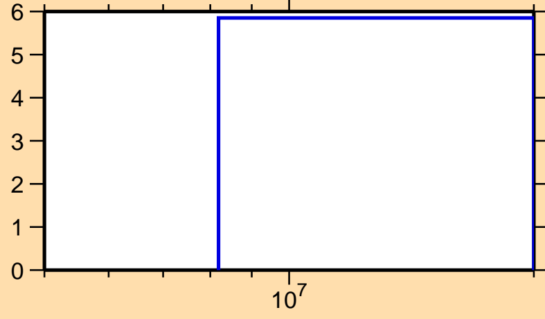
\Delta\sigma/\sigma vs. E for ^{228}\text{Pu}(n,\text{el.})
