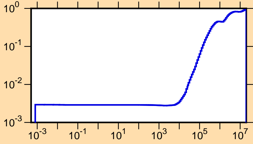
\mu vs. E for ^{229}\text{Pu}(\text{mt251})
