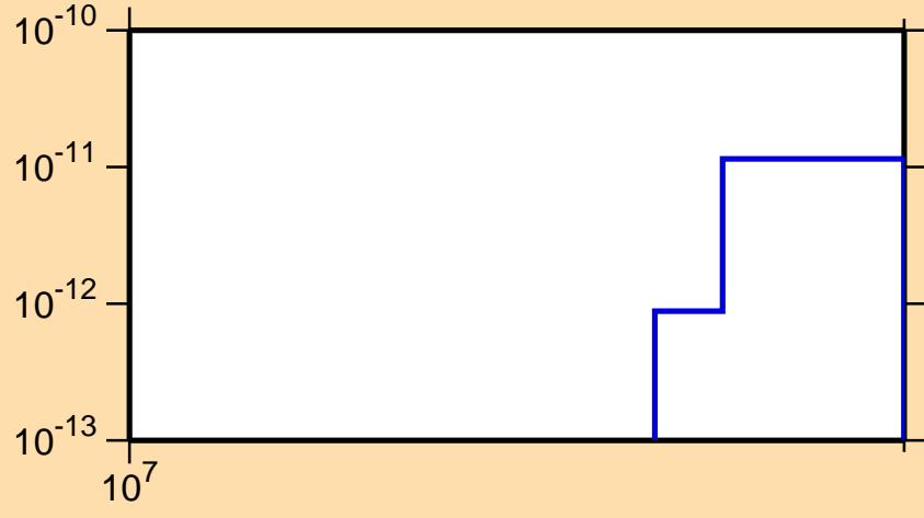
\sigma vs. E for ^{229}\text{Pu}(n,\text{pt})
