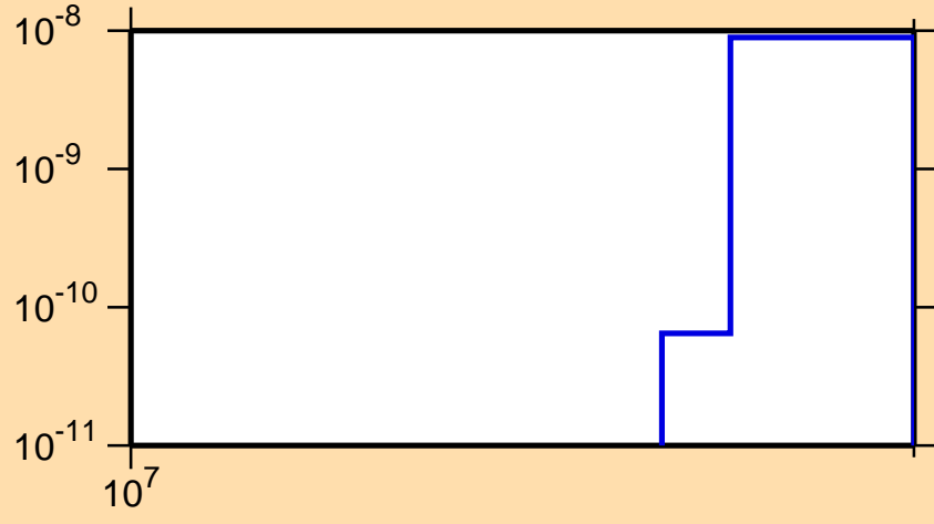
\sigma vs. E for ^{229}\text{Pu}(n,nt)
