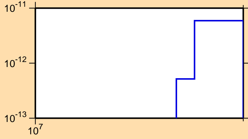
\sigma vs. E for ^{229}\text{Pu}(n,\text{pd})
