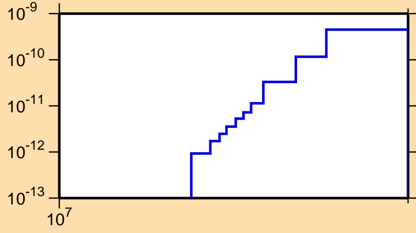
\sigma vs. E for ^{229}\text{Pu}(\text{mt117})
