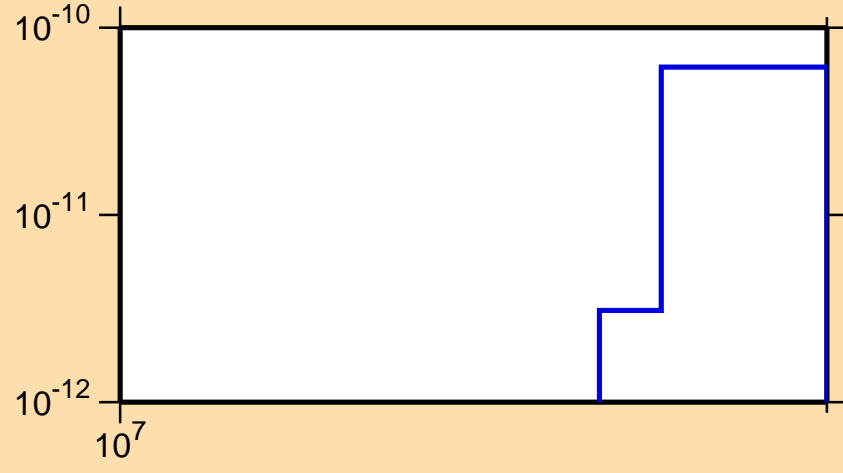
\sigma vs. E for ^{229}\text{Pu} (mt 34)
