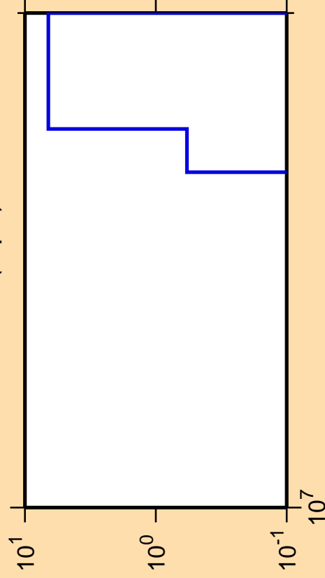
\Delta\sigma/\sigma vs. E for ^{229}\text{Pu}(n,\text{pd})
