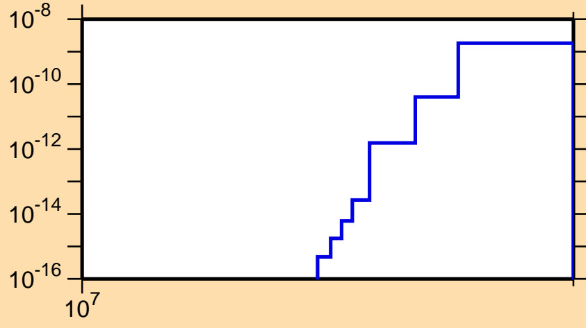
\sigma vs. E for ^{232}\text{Pu}(n,\text{nd})
