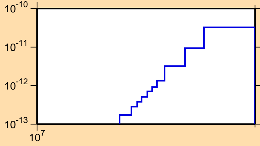
\sigma vs. E for ^{232}\text{Pu}(n,p\alpha)
