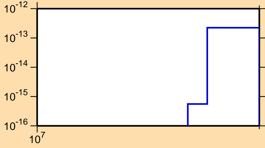
\sigma vs. E for ^{232}\text{Pu}(n,3n\alpha)
