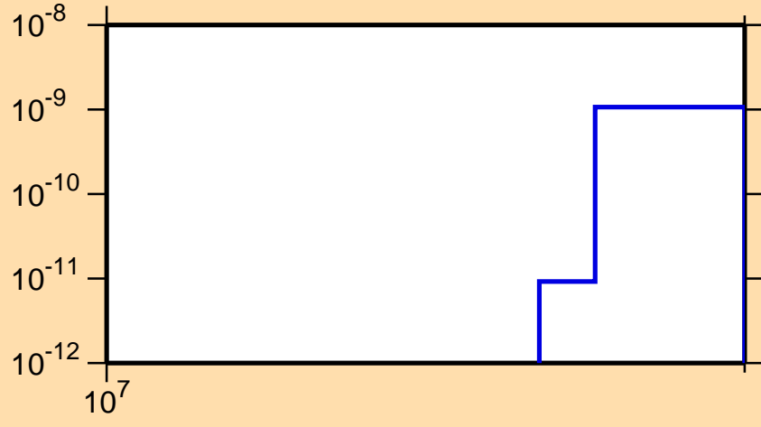
\sigma vs. E for ^{232}\text{Pu}(n,2np)
