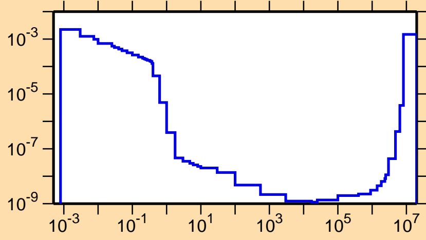
\sigma vs. E for ^{232}\text{Pu}(n,\alpha)
