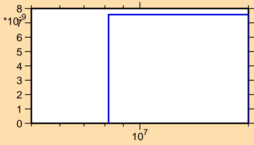
\sigma vs. E for ^{232}\text{Pu}(n,2n\alpha)
