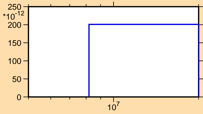
\sigma vs. E for ^{232}\text{Pu}(n,\text{He}3)
