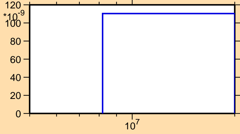
\sigma vs. E for ^{232}\text{Pu}(n,3n)
