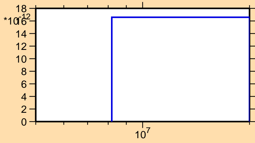
\sigma vs. E for ^{232}\text{Pu}(n,nd)
