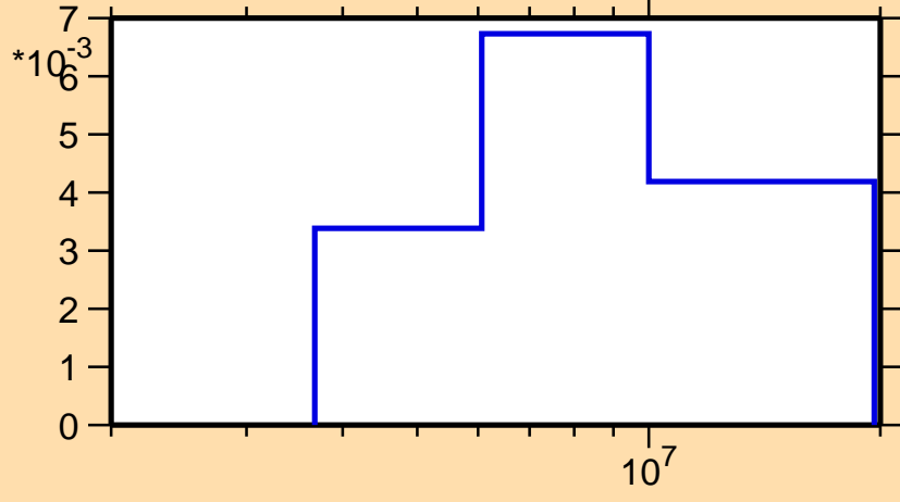
\sigma vs. E for ^{234}\text{Pu}(n,n\text{cont.})
