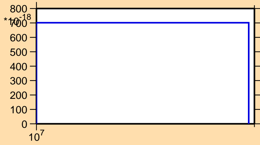
\sigma vs. E for ^{234}\text{Pu}(n,3n\alpha)
