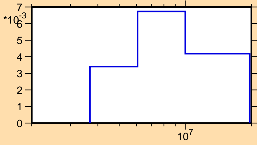
\sigma vs. E for ^{234}\text{Pu}(n,\text{inel.})
