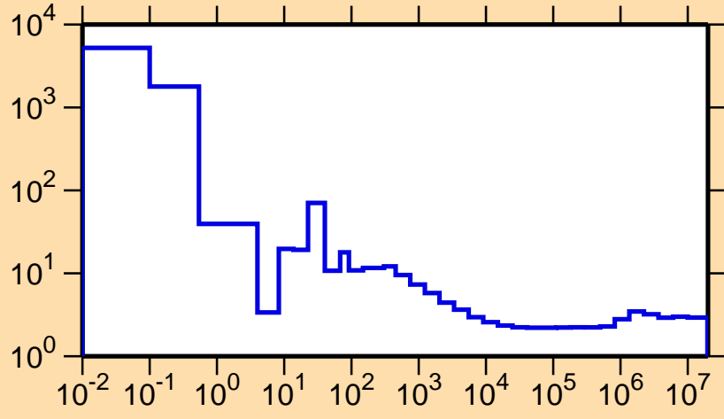
\sigma vs. E for ^{234}\text{Pu}(n,\text{nonel.})
