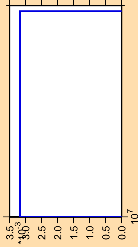
\Delta\sigma/\sigma vs. E for ^{234}\text{Pu}(n,3n\alpha)
