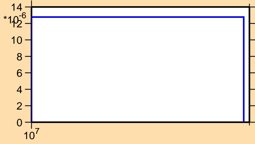
\sigma vs. E for ^{234}\text{Pu}(n,3n)
