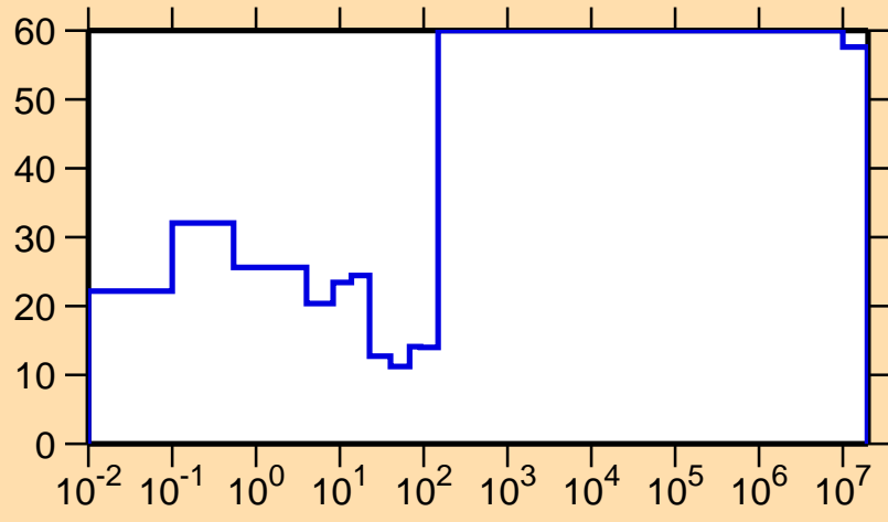
\Delta\sigma/\sigma vs. E for ^{234}\text{Pu}(n,\gamma)
