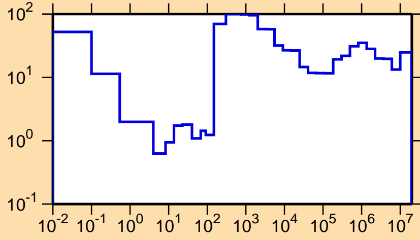
\Delta\sigma/\sigma vs. E for ^{234}\text{Pu}(n,el.)
