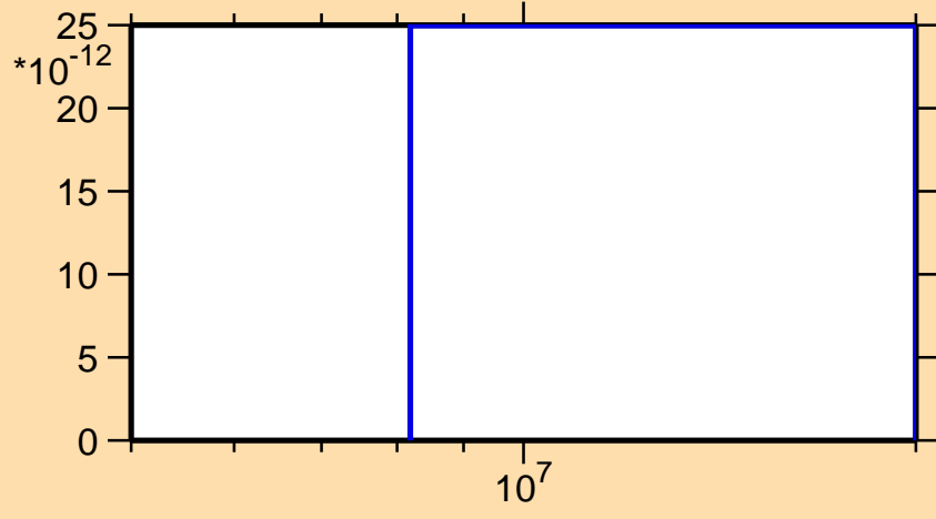
\sigma vs. E for ^{234}\text{Pu}(n,nd)
