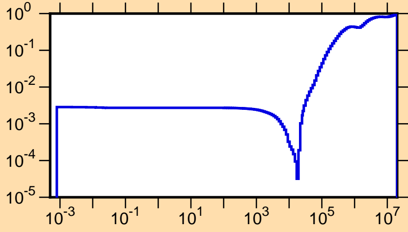
\mu vs. E for ^{235}\text{Pu}(\text{mt251})
