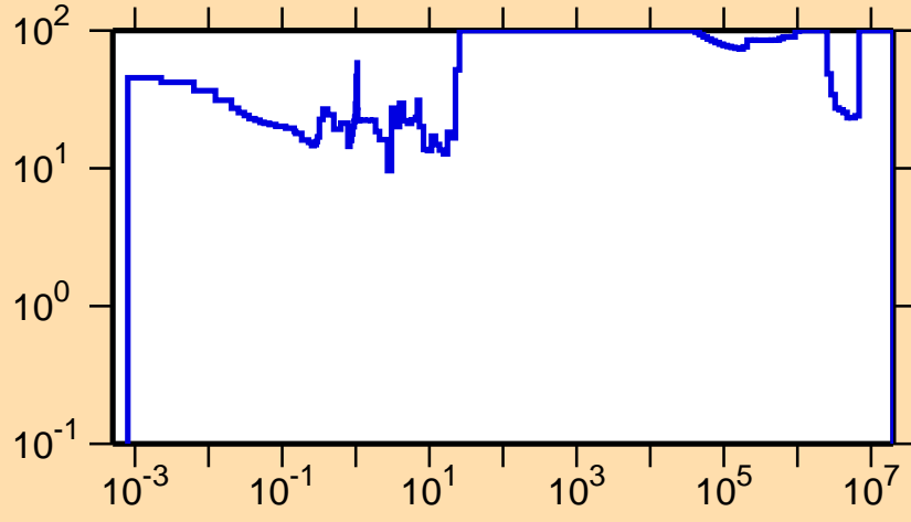
\Delta\sigma/\sigma vs. E for ^{235}\text{Pu}(n,\gamma)
