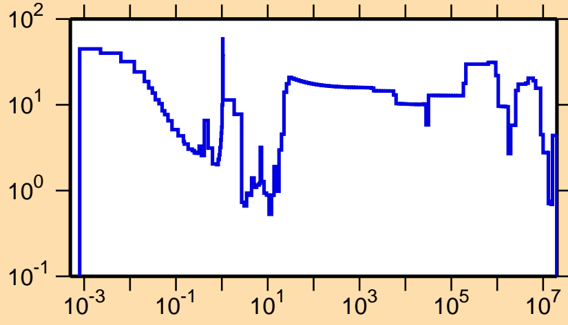
\Delta\sigma/\sigma vs. E for ^{235}\text{Pu}(n,el.)
