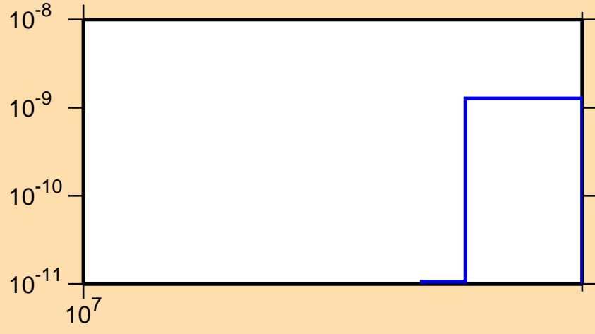
\sigma vs. E for ^{235}\text{Pu}(n,nt)
