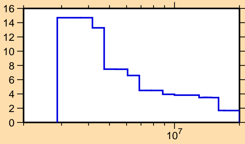
\Delta\sigma/\sigma vs. E for ^{235}\text{Pu}(n,f)
