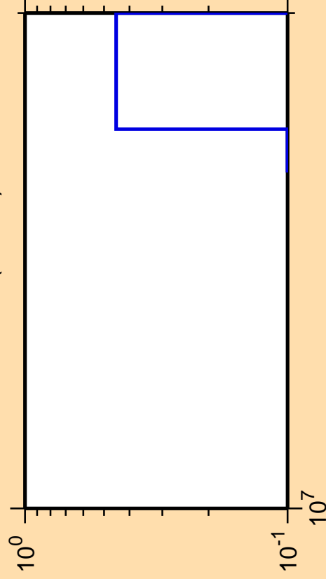
\Delta\sigma/\sigma vs. E for ^{235}\text{Pu} (mt 34)
