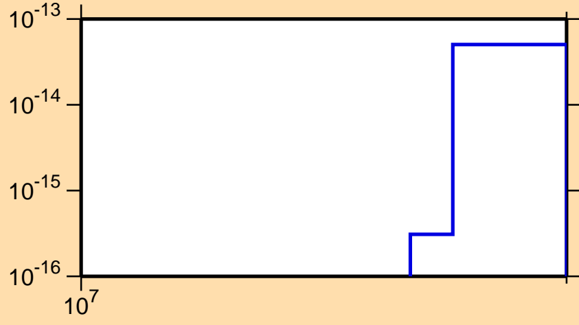
\sigma vs. E for ^{235}\text{Pu} (mt 34)
