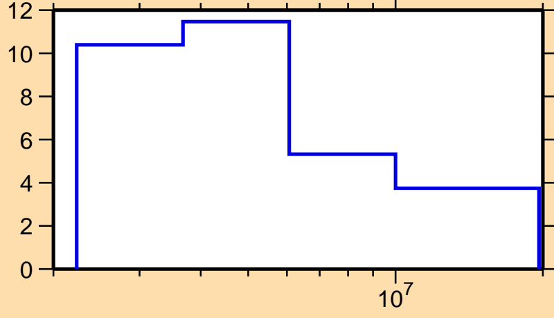
\Delta\sigma/\sigma vs. E for ^{235}\text{Pu}(n,n\text{onel.})
