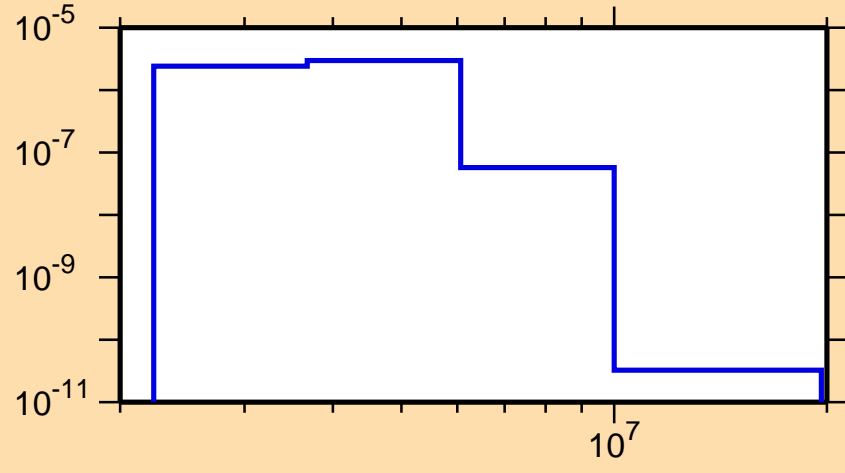
\sigma vs. E for ^{235}\text{Pu}(n,n_1)
