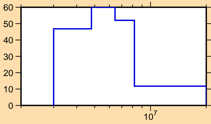
\Delta\sigma/\sigma vs. E for ^{235}\text{Pu}(n,n\text{cont.})
