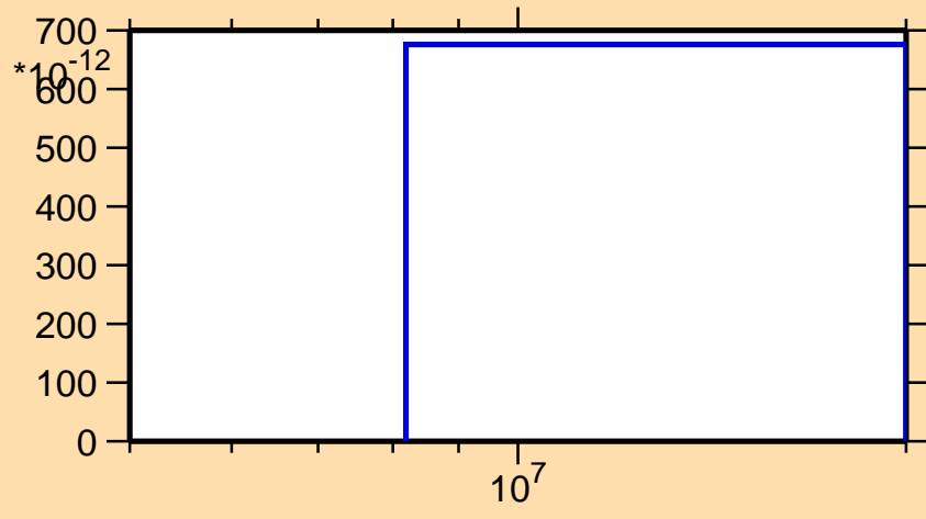
\sigma vs. E for ^{235}\text{Pu}(n,\text{nd})
