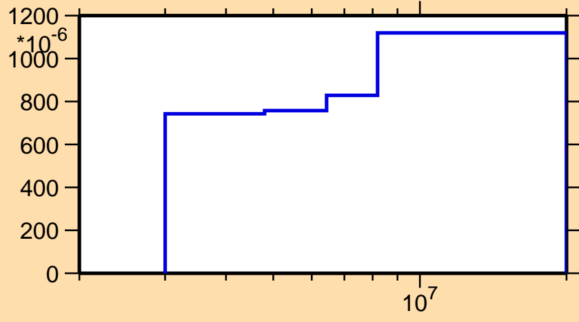
\sigma vs. E for ^{235}\text{Pu}(n,n\text{cont.})
