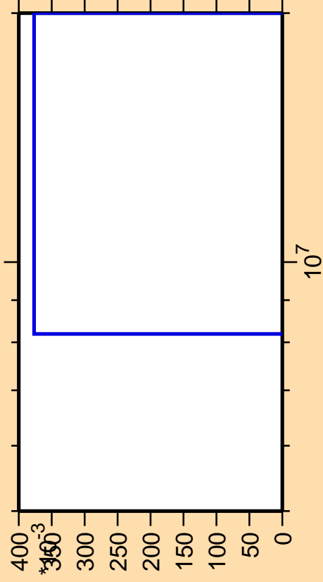
\Delta\sigma/\sigma vs. E for ^{235}\text{Pu}(n,n_2)
