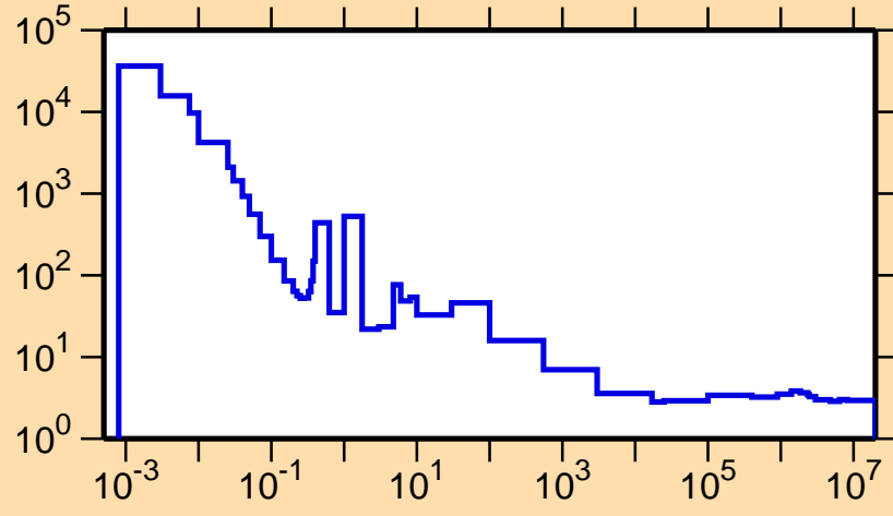
\sigma vs. E for ^{235}\text{Pu}(n,f)
