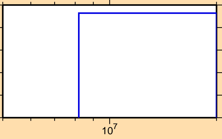
\sigma vs. E for ^{235}\text{Pu}(n,\text{He3})
