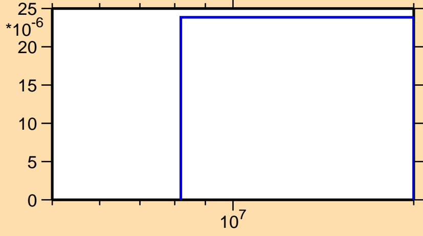
\sigma vs. E for ^{235}\text{Pu}(n,t)
