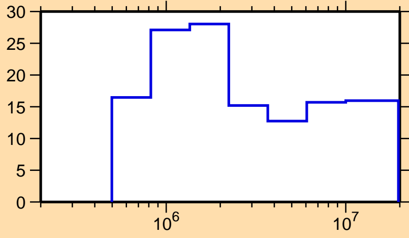
\Delta\sigma/\sigma vs. E for ^{236}\text{Pu}(n,n\text{onel.})
