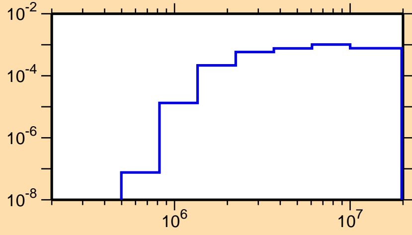
\sigma vs. E for ^{236}\text{Pu}(n,n_4)
