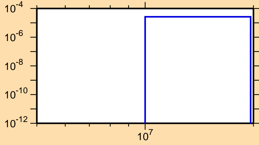
\sigma vs. E for ^{236}\text{Pu}(n,t)
