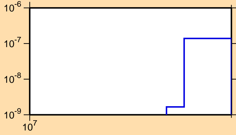
\sigma vs. E for ^{238}\text{Pu}(n,\text{nd})
