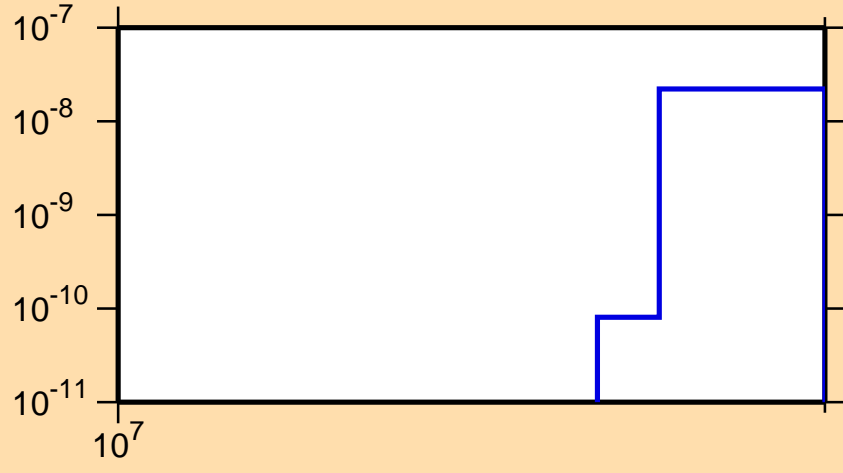
\sigma vs. E for ^{238}\text{Pu}(n,2np)
