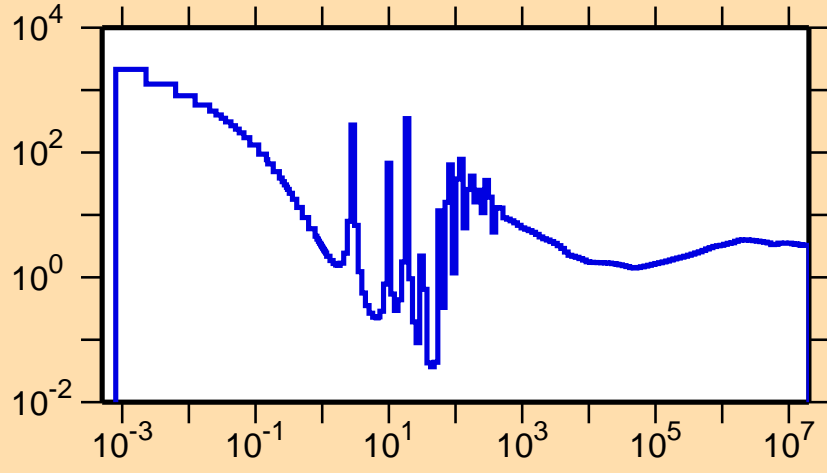
\sigma vs. E for ^{238}\text{Pu}(n,\text{nonel.})
