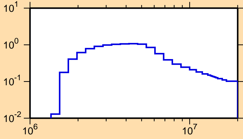
\sigma vs. E for ^{238}\text{Pu}(n,n\text{cont.})
