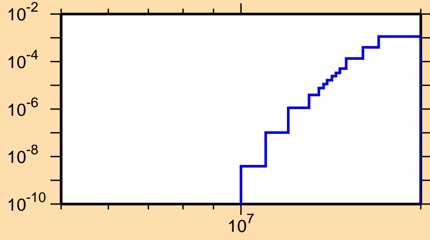
\sigma vs. E for ^{238}\text{Pu}(n,np)
