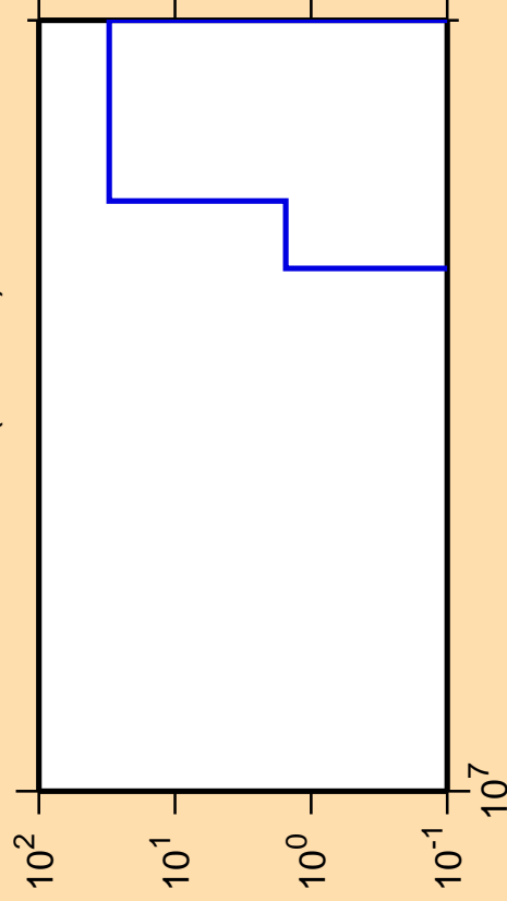
\Delta\sigma/\sigma vs. E for ^{238}\text{Pu}(n,\text{He3})
