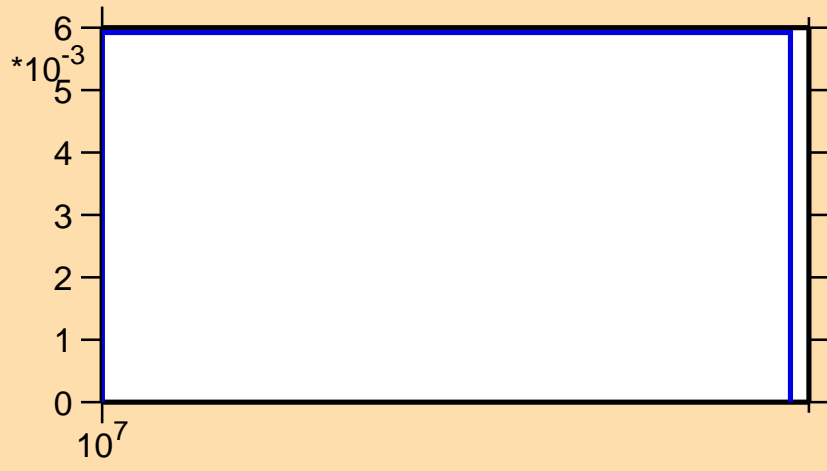
\sigma vs. E for ^{238}\text{Pu}(n,3n)
