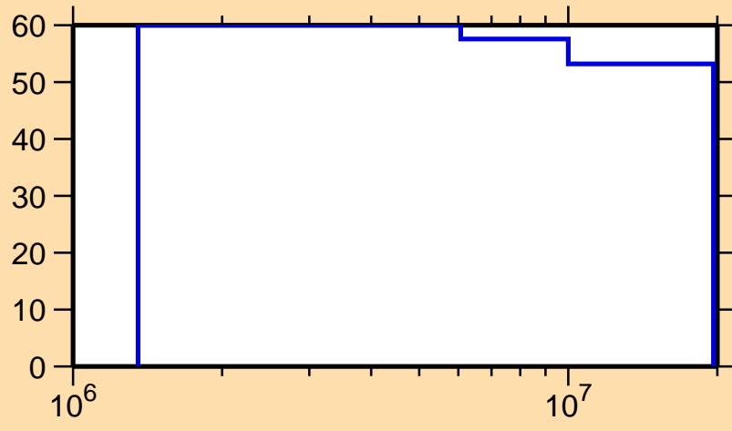
\Delta\sigma/\sigma vs. E for ^{238}\text{Pu}(n,n\text{cont.})
