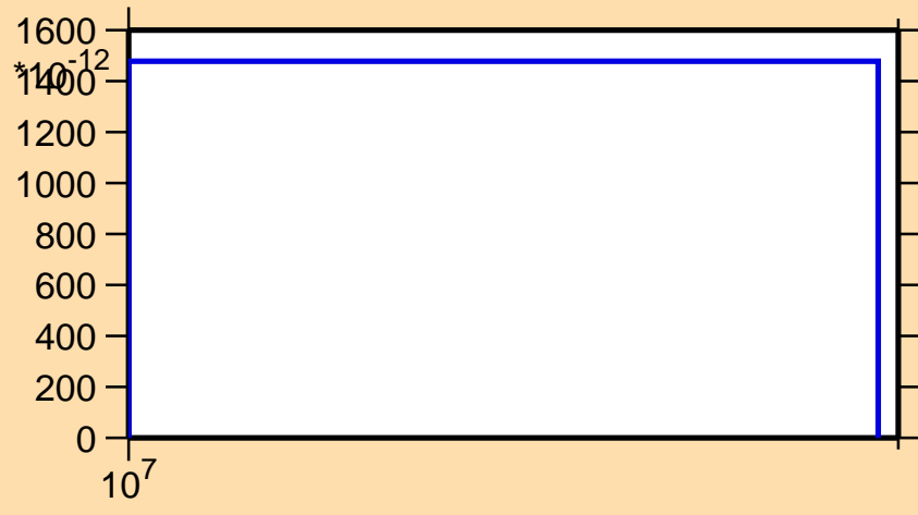
\sigma vs. E for ^{238}\text{Pu}(n,nt)
