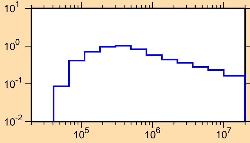
\sigma vs. E for ^{238}\text{Pu}(n,n_1)
