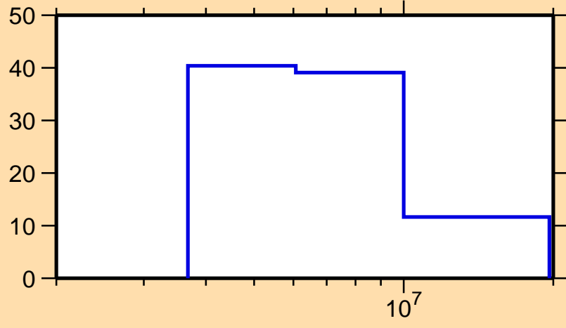
\Delta\sigma/\sigma vs. E for ^{238}\text{Pu}(n,p)
