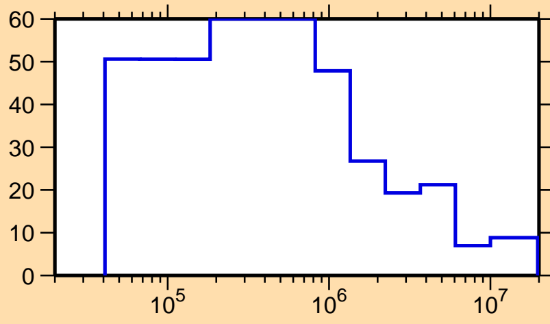
\Delta\sigma/\sigma vs. E for ^{238}\text{Pu}(n,\text{nonel.})
