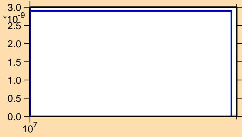
\sigma vs. E for ^{238}\text{Pu}(n,2n\alpha)
