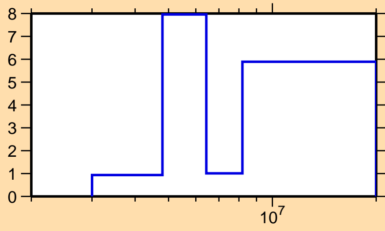
\Delta\sigma/\sigma vs. E for ^{238}\text{Pu}(n,\text{tot.})
