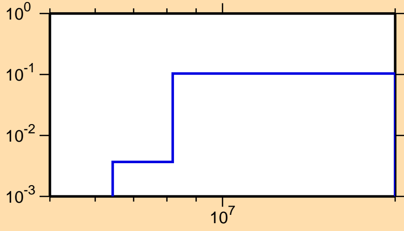
\sigma vs. E for ^{238}\text{Pu}(n,2n)
