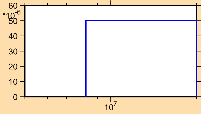
\sigma vs. E for ^{238}\text{Pu}(n,np)
