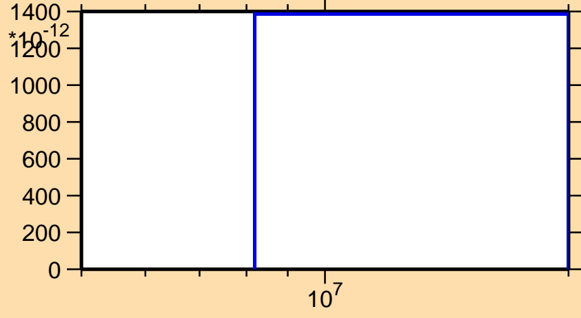
\sigma vs. E for ^{238}\text{Pu}(n,nt)
