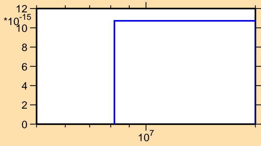
\sigma vs. E for ^{238}\text{Pu}(n,3n\alpha)
