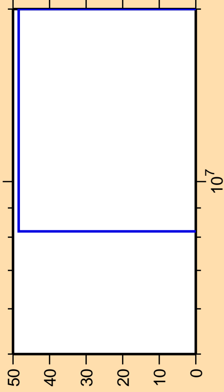
\Delta\sigma/\sigma vs. E for ^{238}\text{Pu}(n,np)
