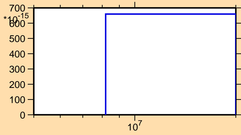
\sigma vs. E for ^{238}\text{Pu}(n,\text{He}3)
