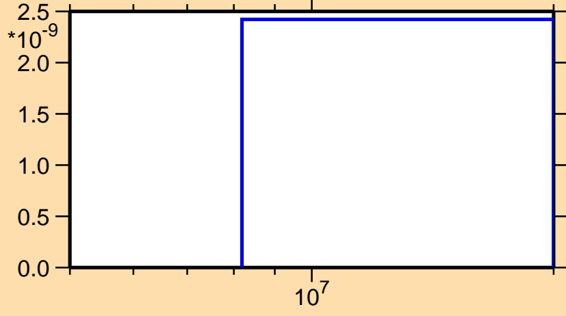
\sigma vs. E for ^{238}\text{Pu}(n,2n\alpha)
