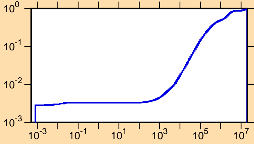
\mu vs. E for ^{241}\text{Pu}(\text{mt251})
