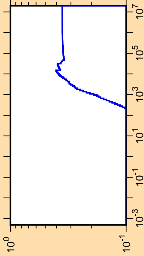
\Delta\mu/\mu vs. E for ^{241}\text{Pu}(\text{mt251})
