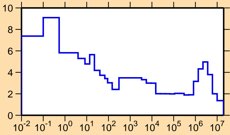
\Delta\sigma/\sigma vs. E for ^{241}\text{Pu}(n,f)
