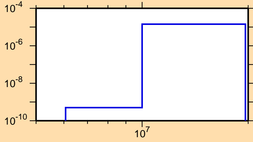
\sigma vs. E for ^{241}\text{Pu}(n,n\alpha)
