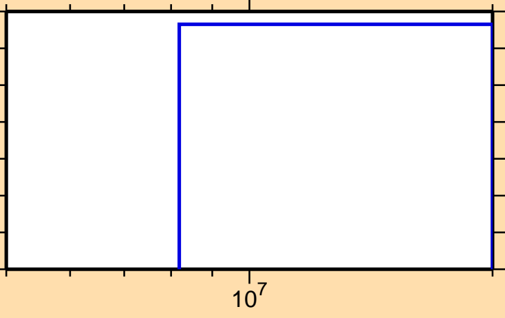
\sigma vs. E for ^{241}\text{Pu}(n,np)
