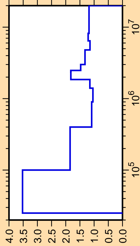
\Delta\sigma/\sigma vs. E for ^{241}\text{Pu}(n,n_1)
