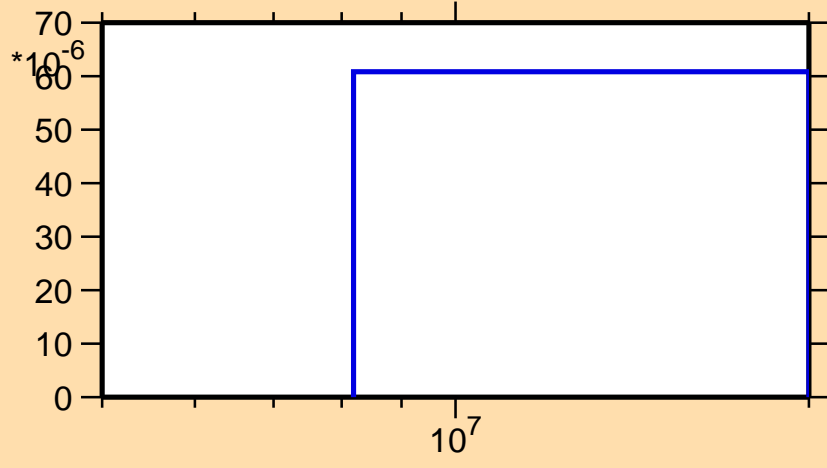
\sigma vs. E for ^{241}\text{Pu}(n,d)
