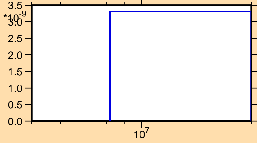
\sigma vs. E for ^{241}\text{Pu}(n,nt)
