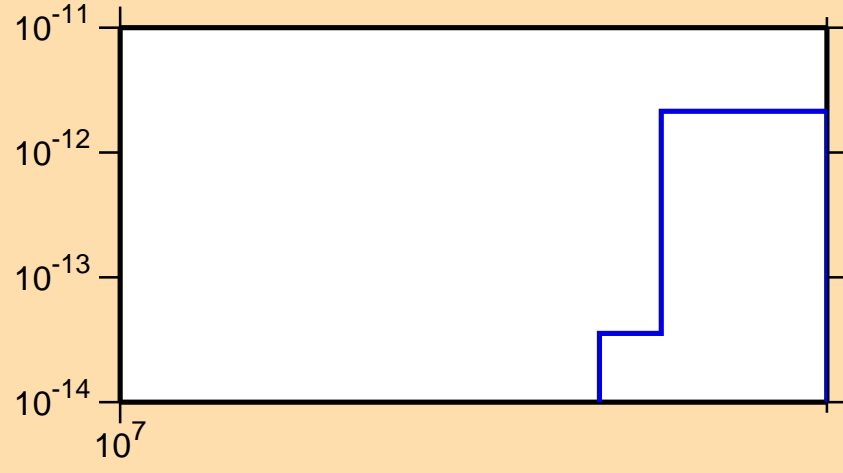
\sigma vs. E for ^{243}\text{Pu}(n,\text{He3})
