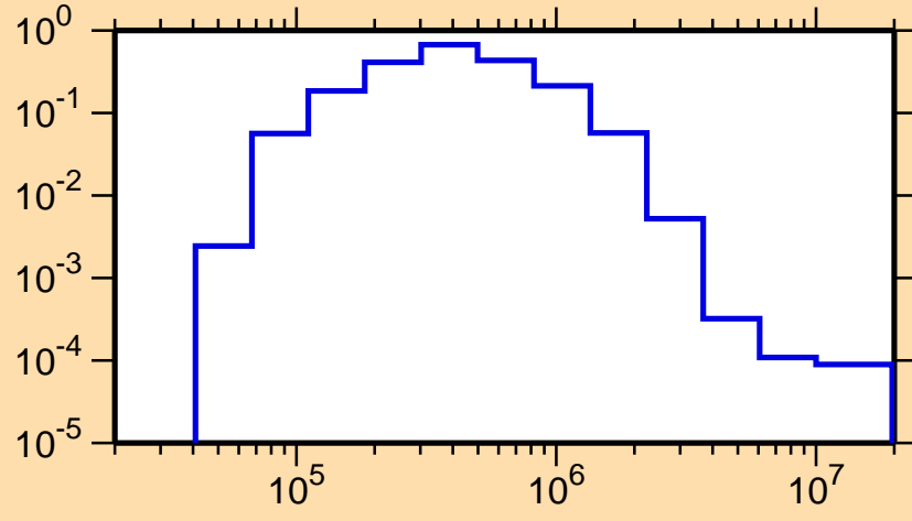
\sigma vs. E for ^{243}\text{Pu}(n,n_1)
