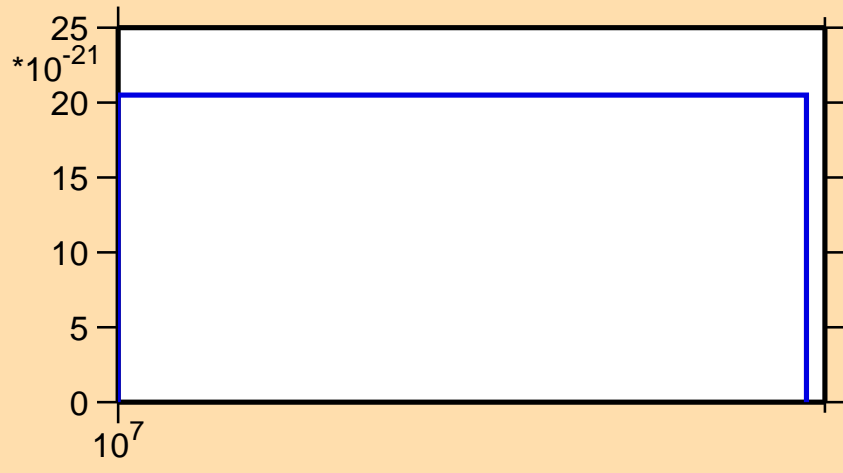
\sigma vs. E for ^{243}\text{Pu} (mt 42)
