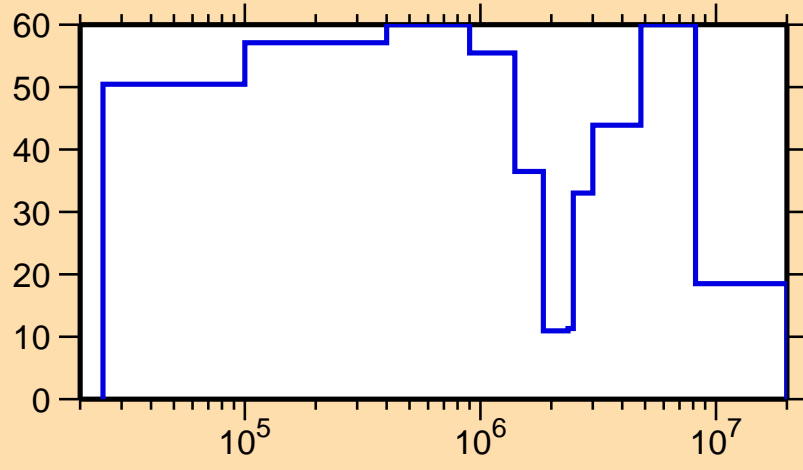
\Delta\sigma/\sigma vs. E for ^{243}\text{Pu}(n,\text{el.})
