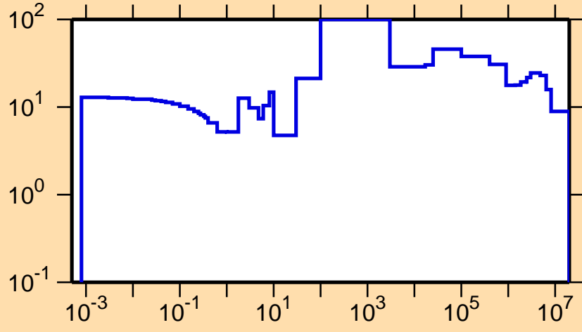
\Delta\sigma/\sigma vs. E for ^{243}\text{Pu}(n,tot.)
