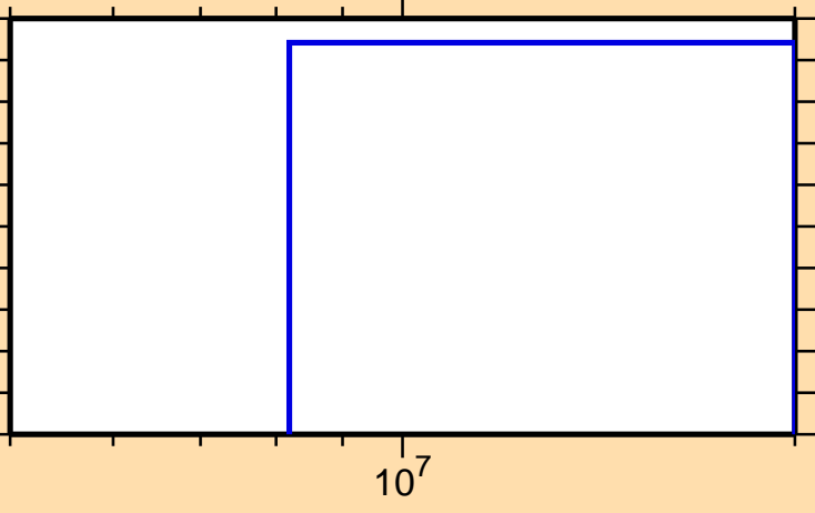
\sigma vs. E for ^{243}\text{Pu}(\text{mt } 42)
