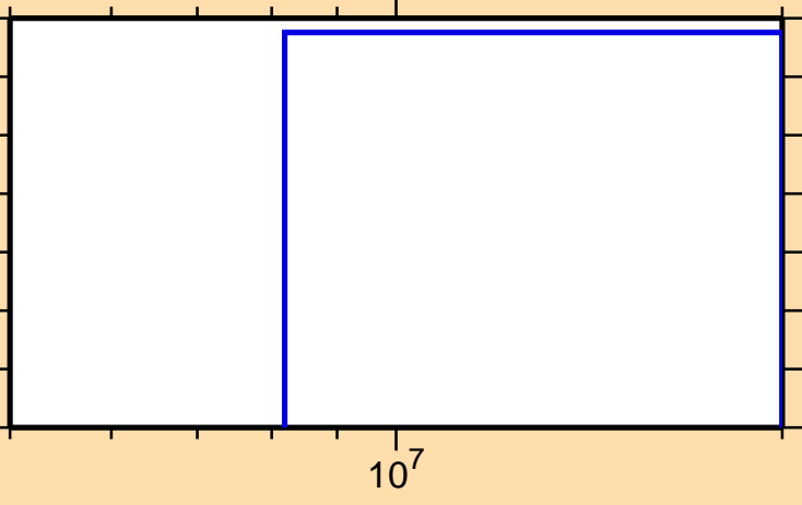
\sigma vs. E for ^{244}\text{Pu}(n,nt)
