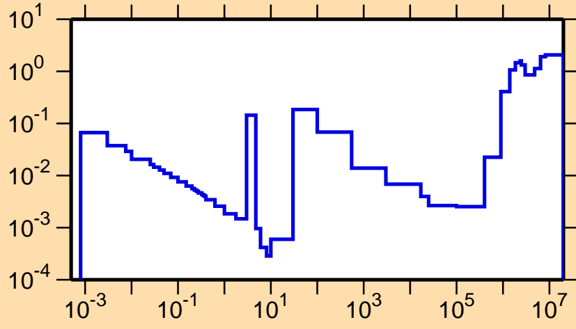
\sigma vs. E for ^{244}\text{Pu}(n,f)
