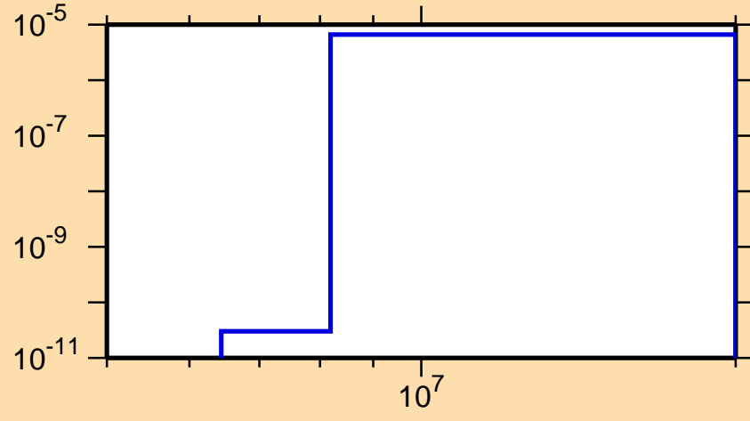
\sigma vs. E for ^{244}\text{Pu}(n,n\alpha)
