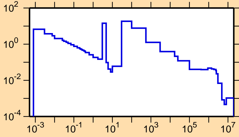
\sigma vs. E for ^{244}\text{Pu}(n,\gamma)
