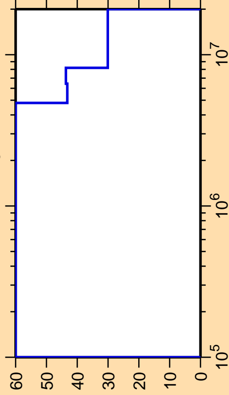
\Delta\sigma/\sigma vs. E for ^{244}\text{Pu}(n,n_3)
