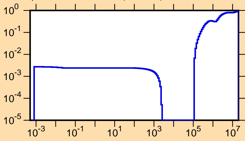
\mu vs. E for ^{245}\text{Pu}(\text{mt251})
