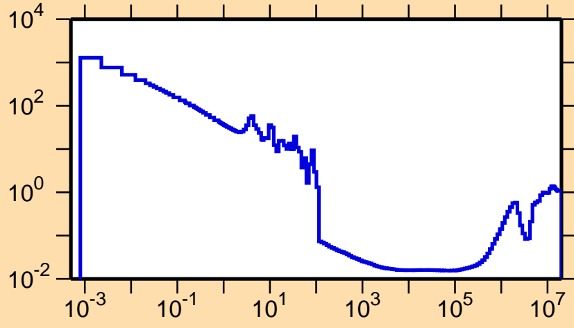
\sigma vs. E for ^{245}\text{Pu}(n,f)
