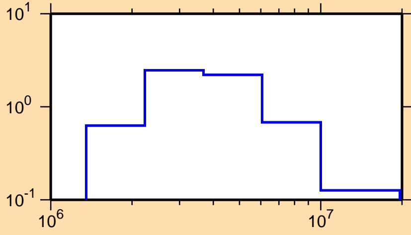
\sigma vs. E for ^{245}\text{Pu}(n,n\text{cont.})
