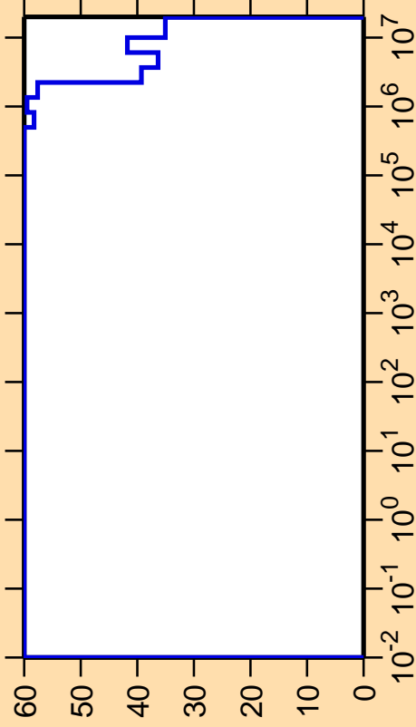
\Delta\sigma/\sigma vs. E for ^{245}\text{Pu}(n,\text{nonel.})
