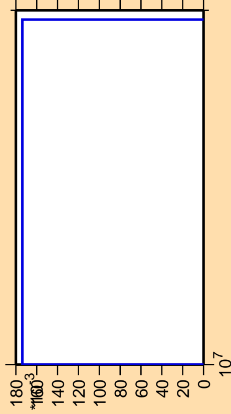
\Delta\sigma/\sigma vs. E for ^{245}\text{Pu}(n,3n\alpha)
