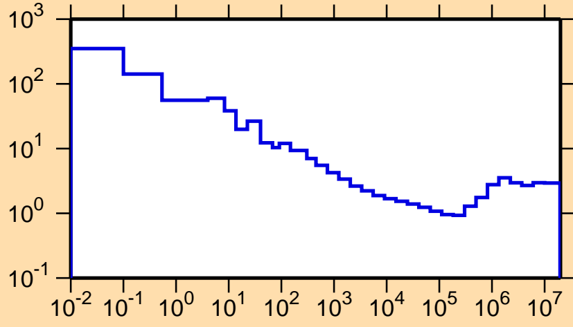
\sigma vs. E for ^{245}\text{Pu}(n,\text{nonel.})
