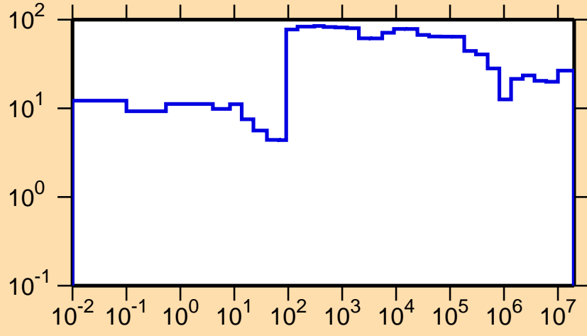
\Delta\sigma/\sigma vs. E for ^{245}\text{Pu}(n,\text{tot.})
