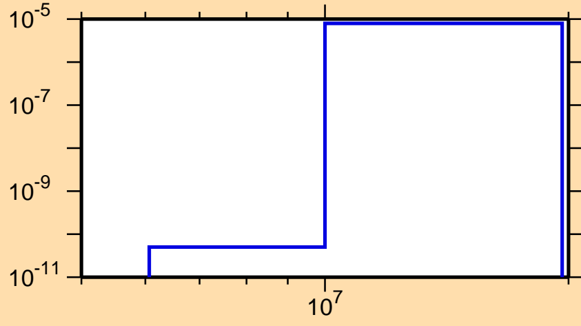
\sigma vs. E for ^{245}\text{Pu}(n,n\alpha)
