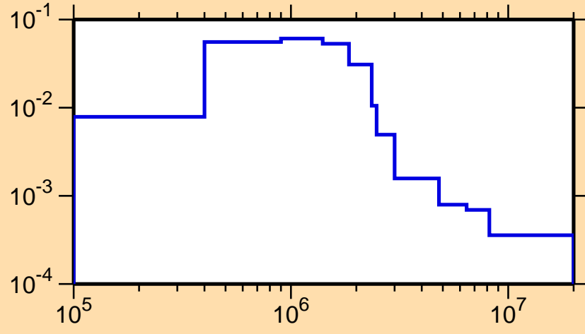
\sigma vs. E for ^{245}\text{Pu}(n,n_4)
