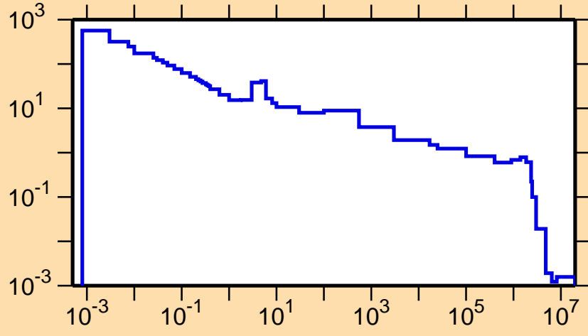
\sigma vs. E for ^{245}\text{Pu}(n,\gamma)
