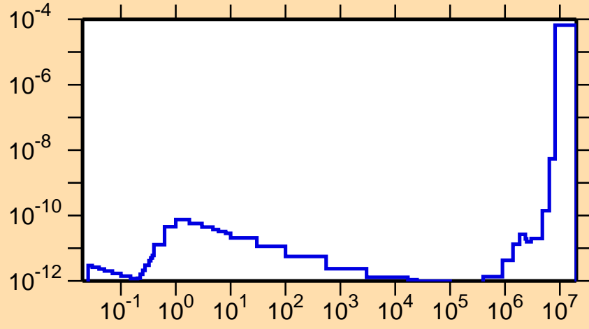
\sigma vs. E for ^{245}\text{Pu}(n,\alpha)
