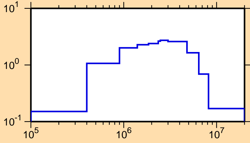
\sigma vs. E for ^{245}\text{Pu}(n,\text{inel.})
