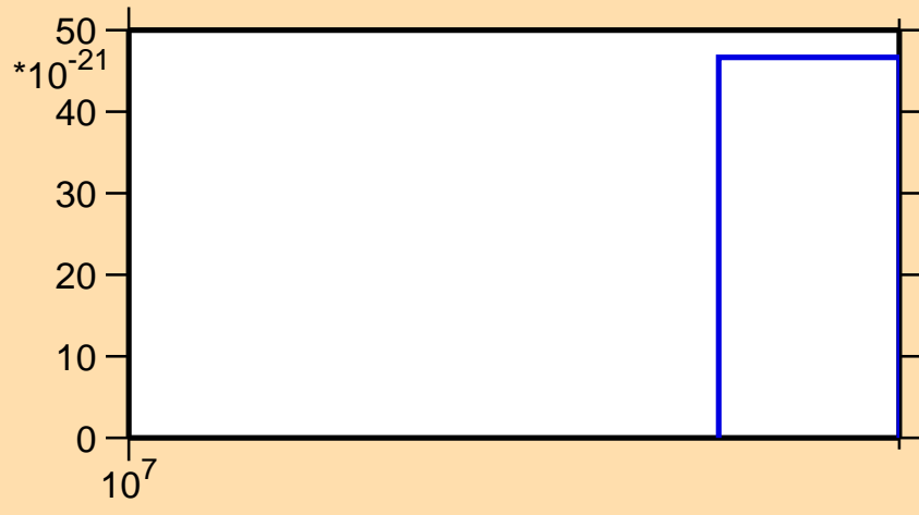
\sigma vs. E for ^{208}\text{Ra}(\text{mt } 11)
