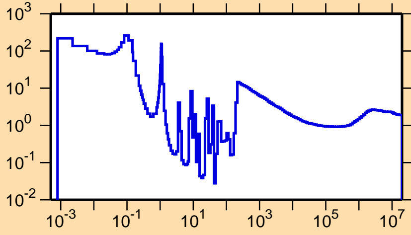
\sigma vs. E for ^{208}\text{Ra}(n,\text{nonel.})
