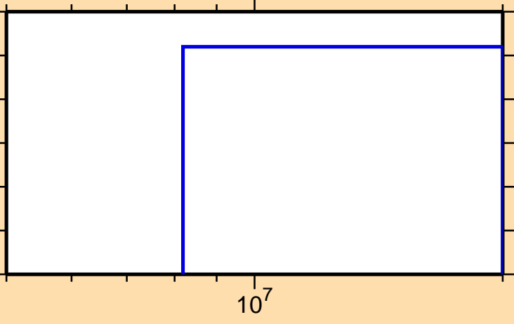
\sigma vs. E for ^{208}\text{Ra}(n,t)
