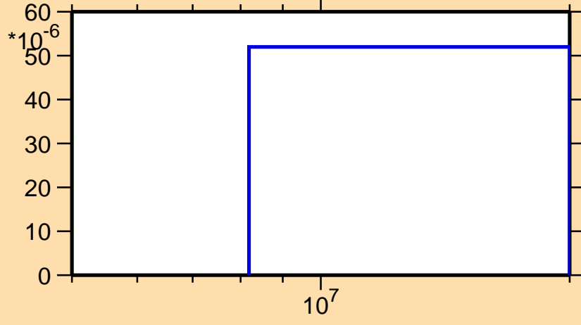
\sigma vs. E for ^{208}\text{Ra}(n,t)
