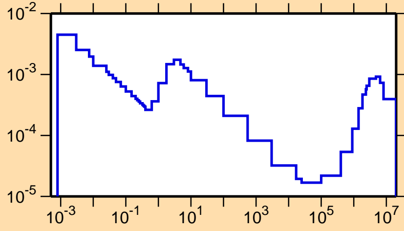
\sigma vs. E for ^{208}\text{Ra}(n,p\alpha)
