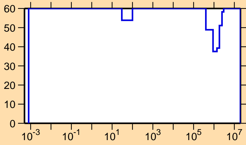
\Delta\sigma/\sigma vs. E for ^{208}\text{Ra}(n,\gamma)
