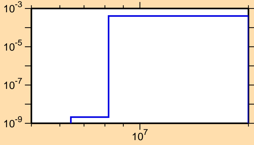
\sigma vs. E for ^{208}\text{Ra}(\text{mt } 45)
