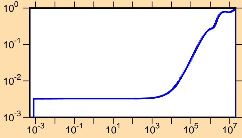
\mu vs. E for ^{209}\text{Ra}(\text{mt251})
