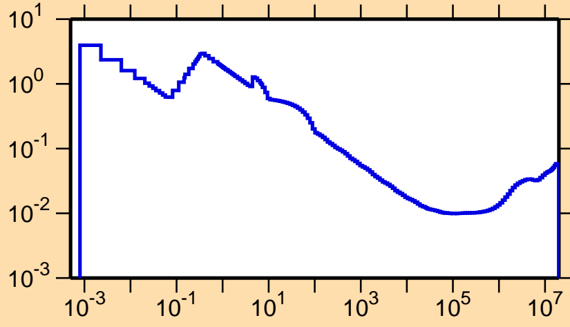
\sigma vs. E for ^{209}\text{Ra}(n,p)
