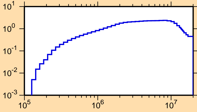
\sigma vs. E for ^{209}\text{Ra}(n,\text{inel.})
