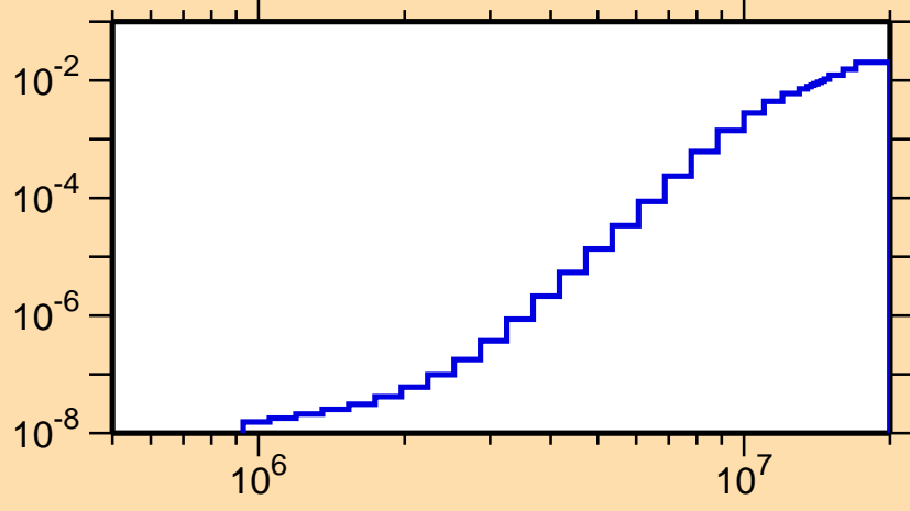
\sigma vs. E for ^{209}\text{Ra}(n,n\alpha)
