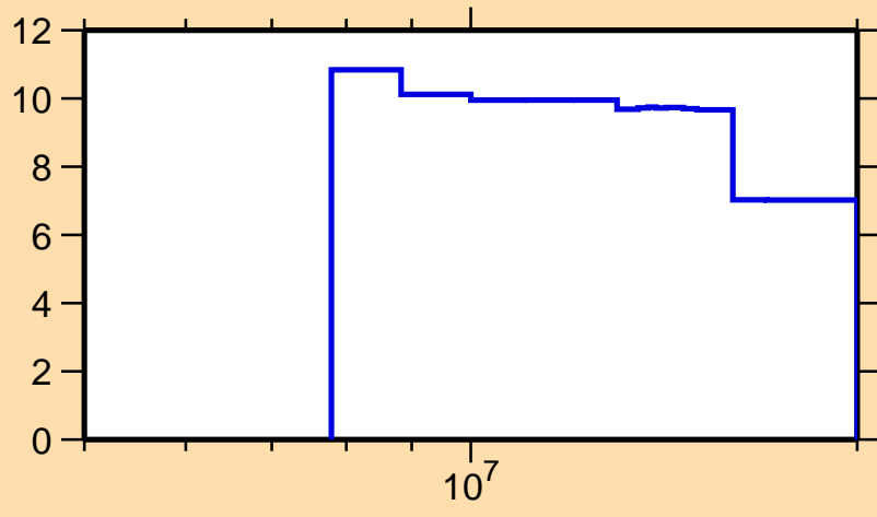
\Delta\sigma/\sigma vs. E for ^{209}\text{Ra}(n,\text{nonel.})
