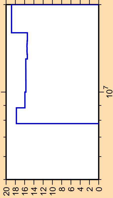
\Delta\sigma/\sigma vs. E for ^{209}\text{Ra}(n,n_1)
