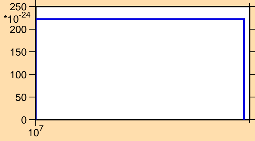
\sigma vs. E for ^{209}\text{Ra}(\text{mt 11})
