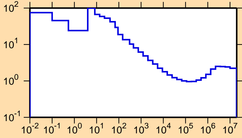
\sigma vs. E for ^{209}\text{Ra}(n,\text{nonel.})
