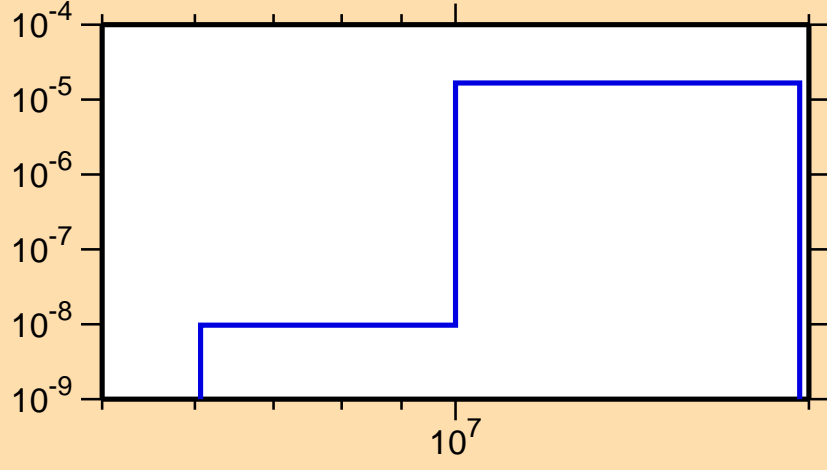
\sigma vs. E for ^{209}\text{Ra}(\text{mt } 45)
