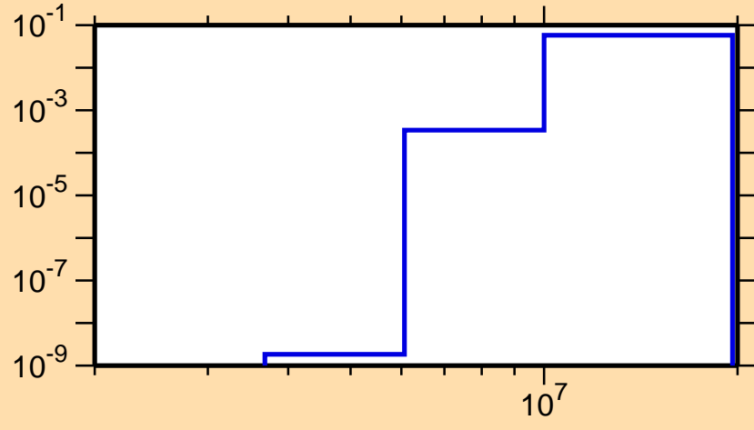
\sigma vs. E for ^{209}\text{Ra}(n,np)
