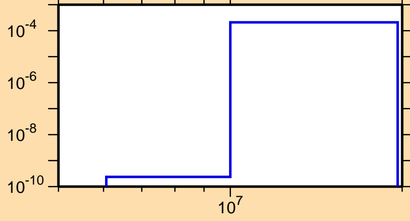
\sigma vs. E for ^{209}\text{Ra}(n,t)
