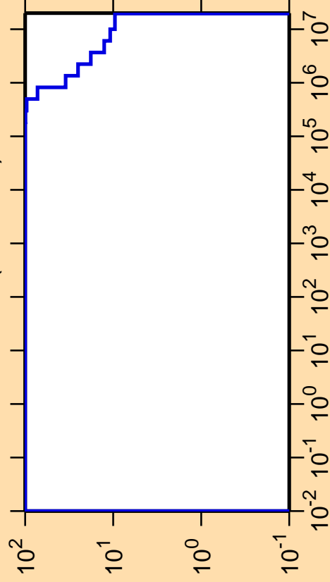
\Delta\sigma/\sigma vs. E for ^{209}\text{Ra}(n,\text{nonel.})
