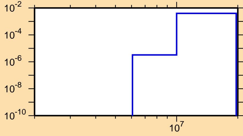
\sigma vs. E for ^{209}\text{Ra}(n,d)
