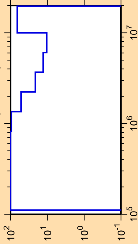
\Delta\sigma/\sigma vs. E for ^{209}\text{Ra}(n,\text{ncont.})
