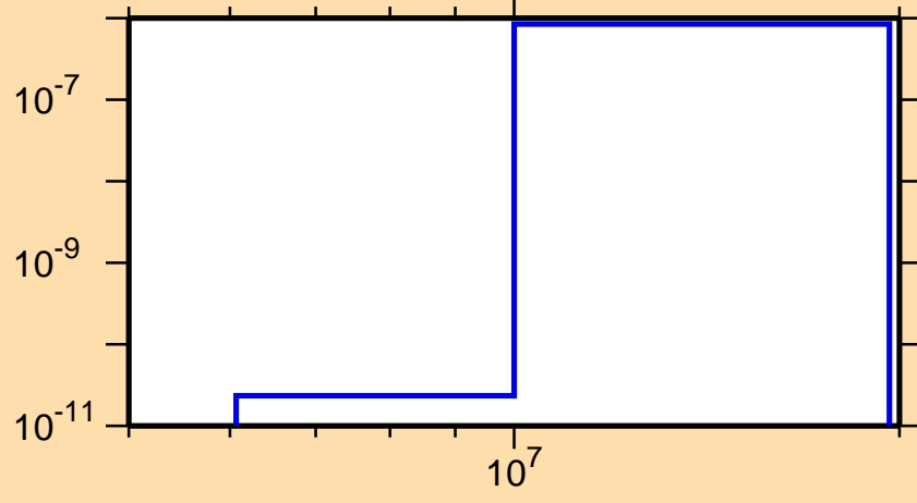
\sigma vs. E for ^{209}\text{Ra}(\text{mt117})
