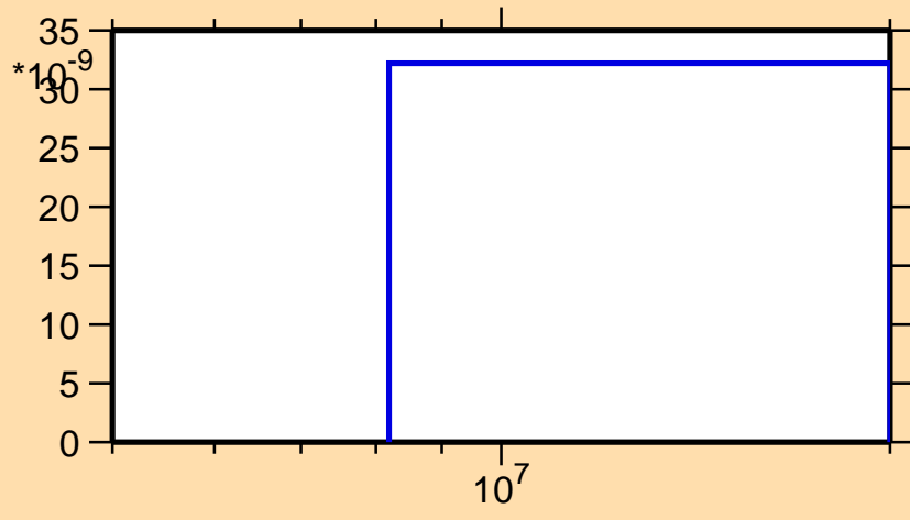
\sigma vs. E for ^{209}\text{Ra}(n,\text{pd})
