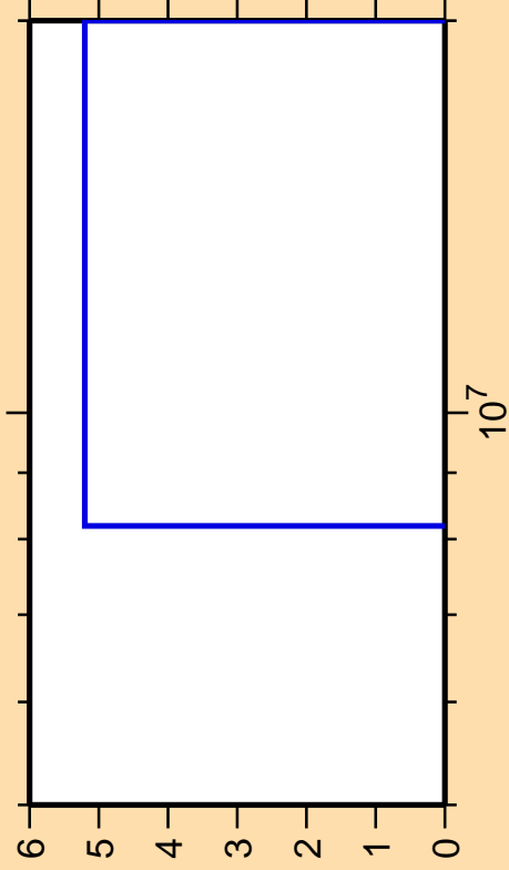
\Delta\sigma/\sigma vs. E for ^{209}\text{Ra}(n,3n\alpha)
