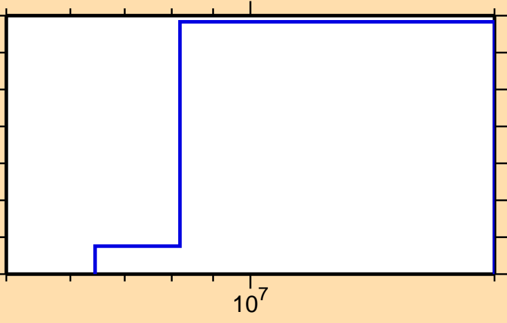
\sigma vs. E for ^{209}\text{Ra}(\text{mt117})
