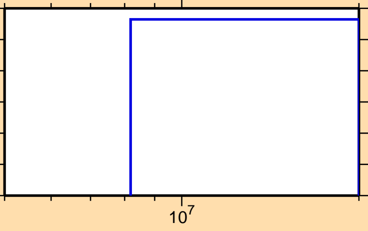
\sigma vs. E for ^{209}\text{Ra}(n,\text{nd})
