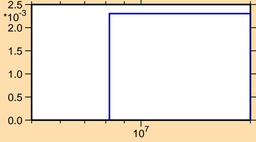
\sigma vs. E for ^{209}\text{Ra}(n,2n\alpha)
