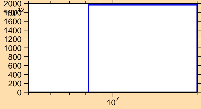
\sigma vs. E for ^{209}\text{Ra}(n,\text{pt})
