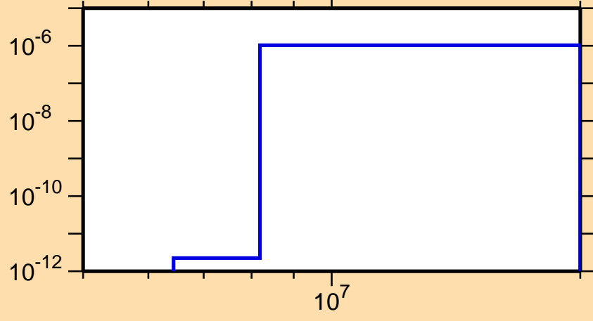
\sigma vs. E for ^{209}\text{Ra}(n,\text{He3})
