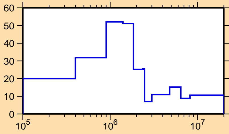
\Delta\sigma/\sigma vs. E for ^{209}\text{Ra}(n, el.)
