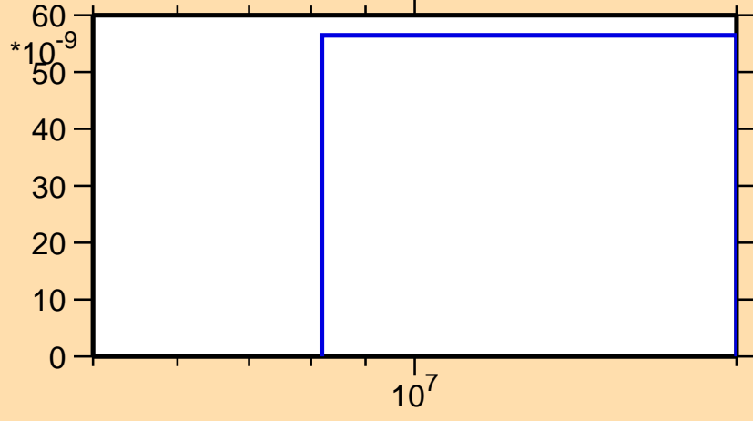
\sigma vs. E for ^{209}\text{Ra}(n,\text{nd})
