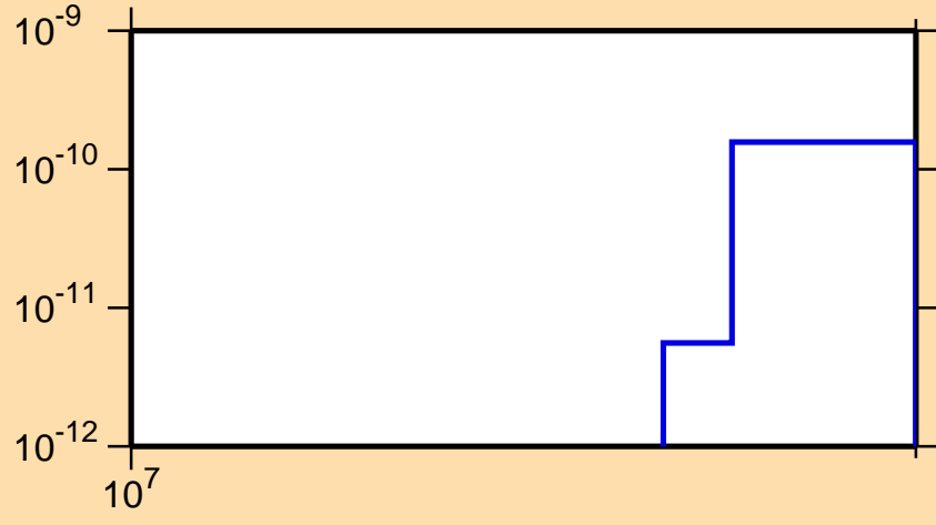
\sigma vs. E for ^{210}\text{Ra}(\text{mt } 34)
