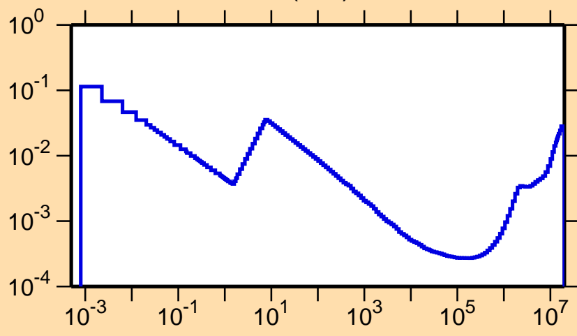
\sigma vs. E for ^{210}\text{Ra}(n,\alpha)
