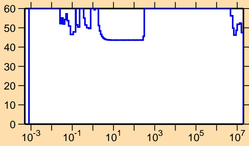
\Delta\sigma/\sigma vs. E for ^{210}\text{Ra}(n,p)
