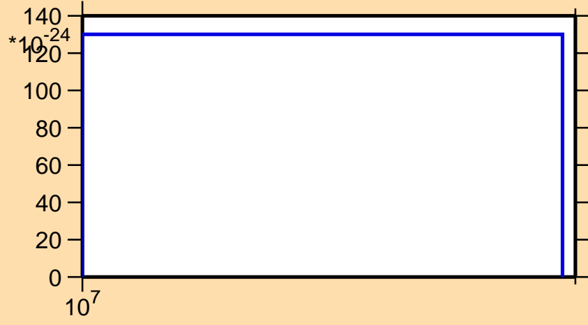
\sigma vs. E for ^{210}\text{Ra} (mt 11)
