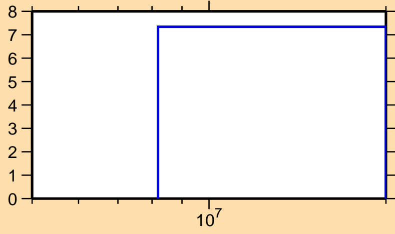
\Delta\sigma/\sigma vs. E for ^{210}\text{Ra}(n,\text{nonel.})
