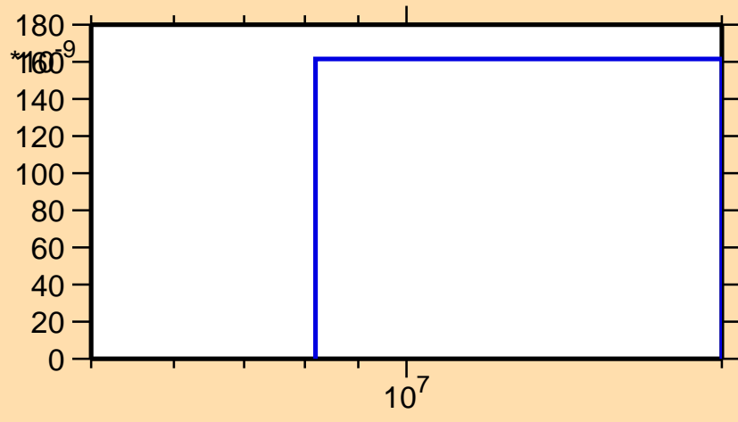
\sigma vs. E for ^{210}\text{Ra}(n,\text{He}3)
