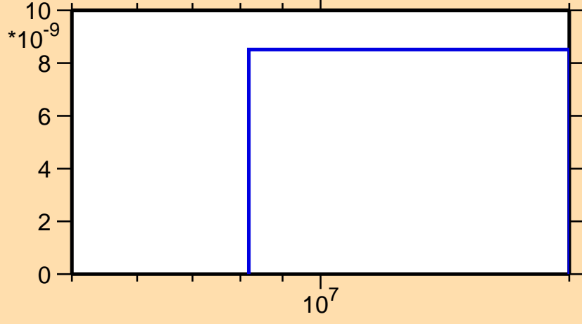
\sigma vs. E for ^{210}\text{Ra}(n,\text{pd})
