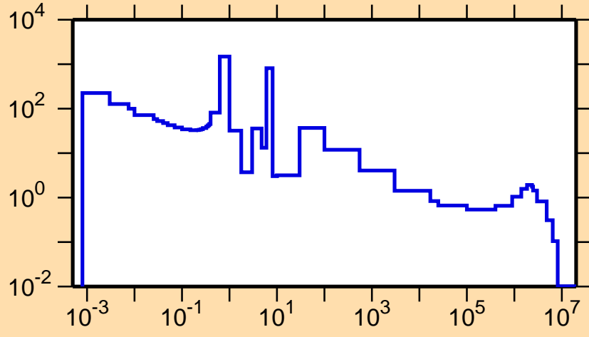
\sigma vs. E for ^{210}\text{Ra}(n,\gamma)
