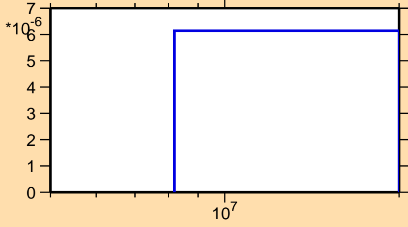
\sigma vs. E for ^{210}\text{Ra}(n,3n)
