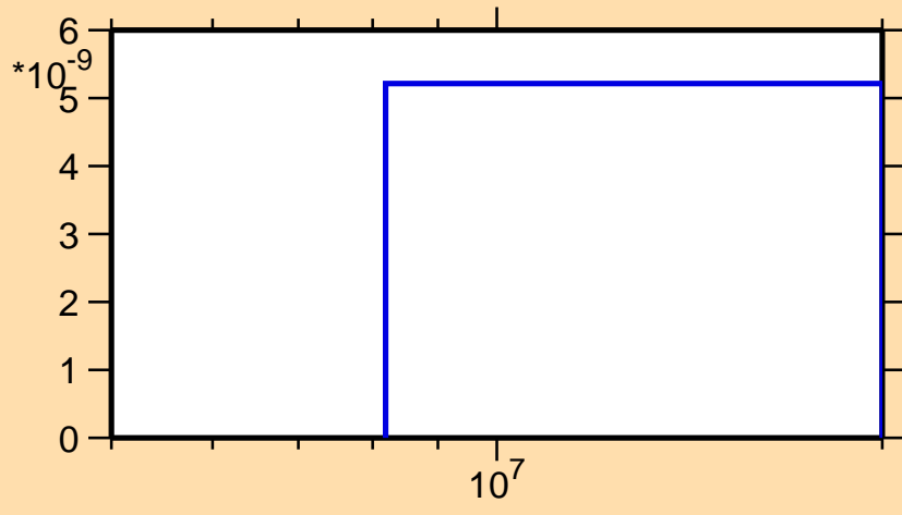
\sigma vs. E for ^{210}\text{Ra}(n,\text{nd})
