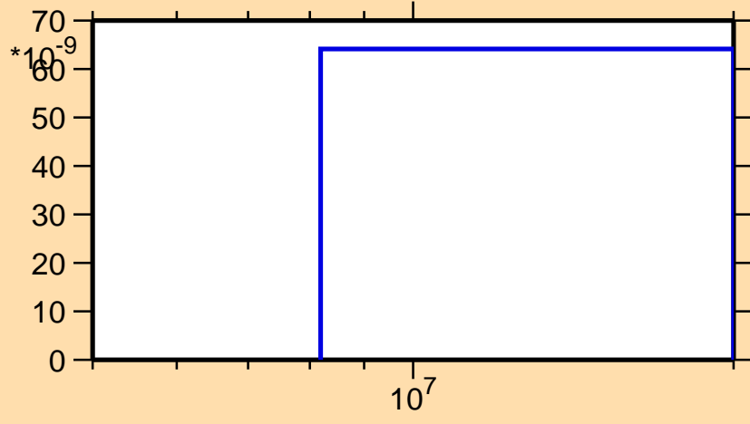
\sigma vs. E for ^{210}\text{Ra}(\text{mt } 45)
