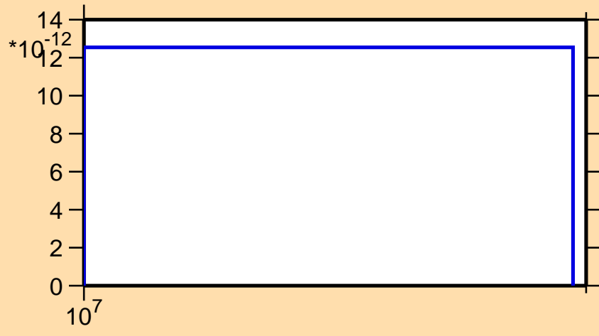
\sigma vs. E for ^{211}\text{Ra} (mt 34)
