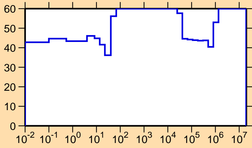
\Delta\sigma/\sigma vs. E for ^{211}\text{Ra}(n,\gamma)
