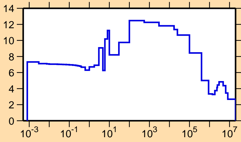
\sigma vs. E for ^{211}\text{Ra}(n,\text{el.})
