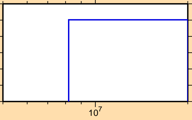
\sigma vs. E for ^{211}\text{Ra}(\text{mt117})
