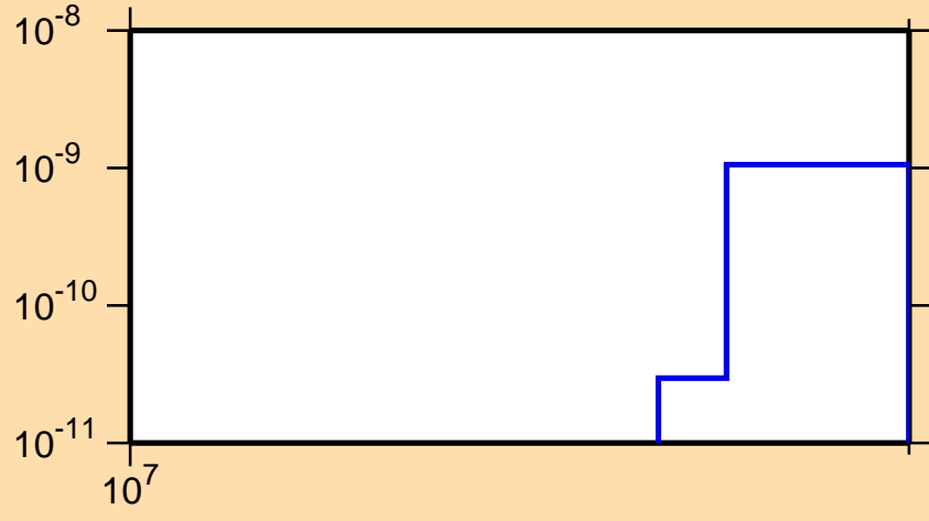
\sigma vs. E for ^{212}\text{Ra}(n,\text{pt})
