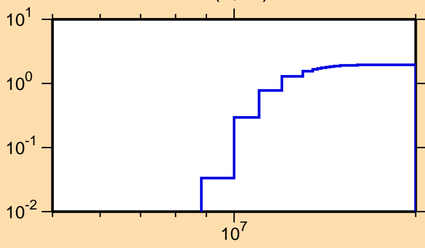
\sigma vs. E for ^{212}\text{Ra}(n,2n)
