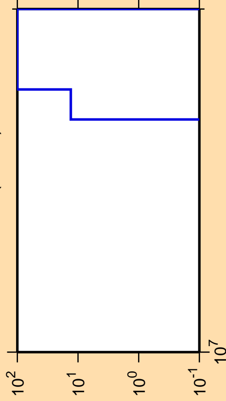
\Delta\sigma/\sigma vs. E for ^{212}\text{Ra} (mt 34)
