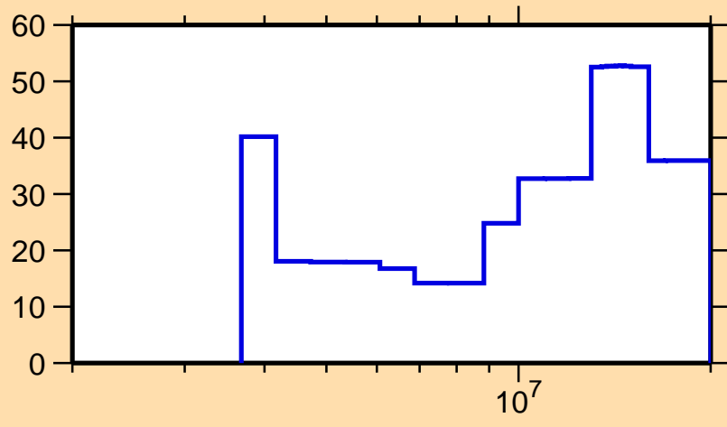
\Delta\sigma/\sigma vs. E for ^{212}\text{Ra}(n,n\text{cont.})
