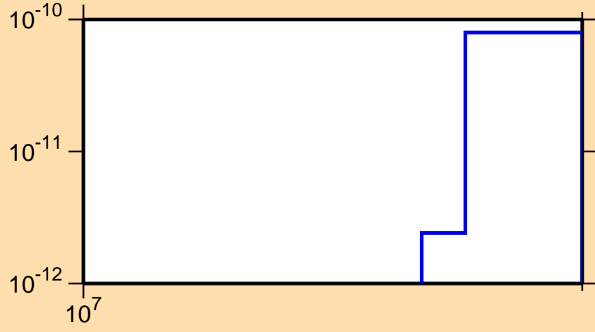
\sigma vs. E for ^{212}\text{Ra} (mt 34)
