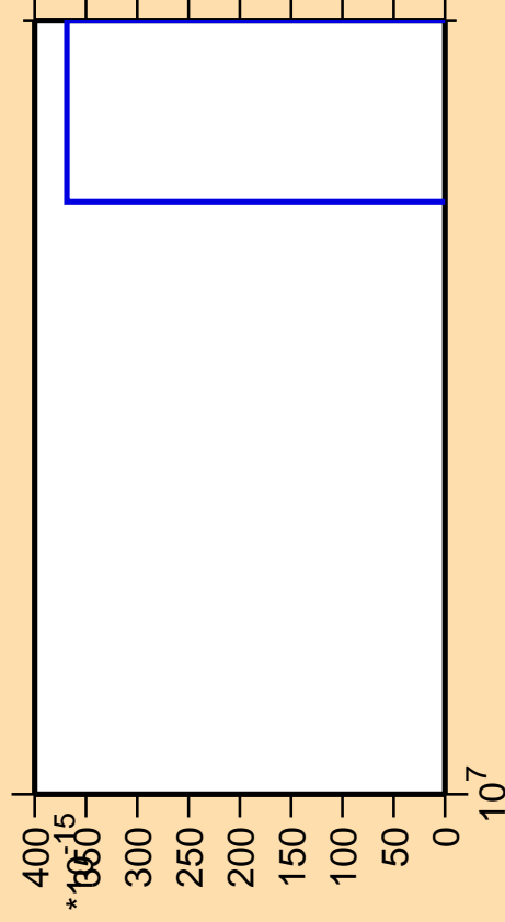
\Delta\sigma/\sigma vs. E for ^{212}\text{Ra} (mt 42)
