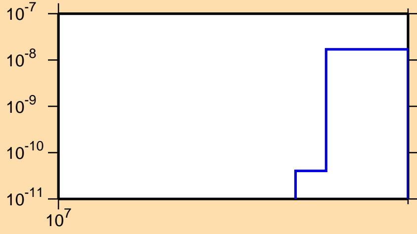
\sigma vs. E for ^{212}\text{Ra}(n,nt)
