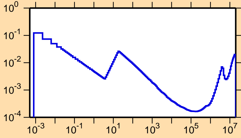
\sigma vs. E for ^{212}\text{Ra}(n,\alpha)
