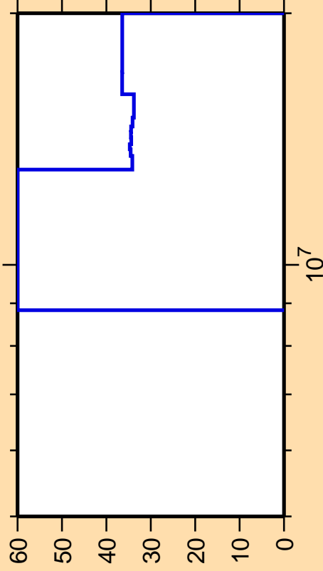
\Delta\sigma/\sigma vs. E for ^{212}\text{Ra}(n,p)
