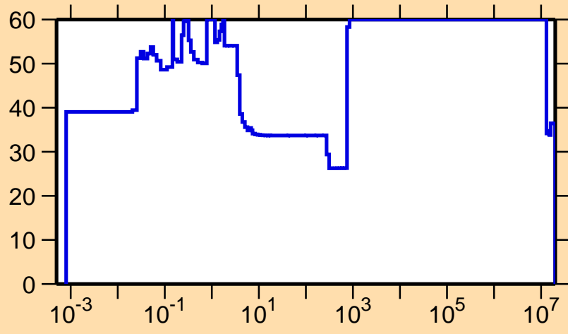
\Delta\sigma/\sigma vs. E for ^{212}\text{Ra}(n,p)
