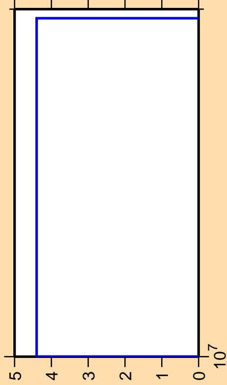
\Delta\sigma/\sigma vs. E for ^{212}\text{Ra} (mt 34)
