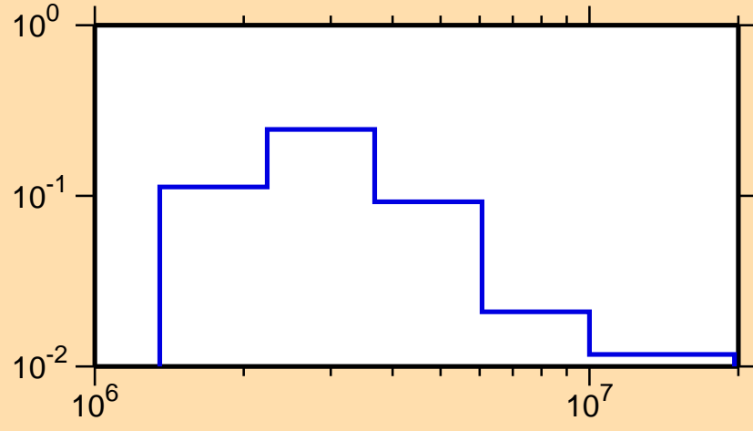
\sigma vs. E for ^{212}\text{Ra}(n,n_2)
