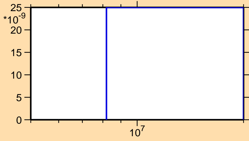
\sigma vs. E for ^{212}\text{Ra} (mt 45)
