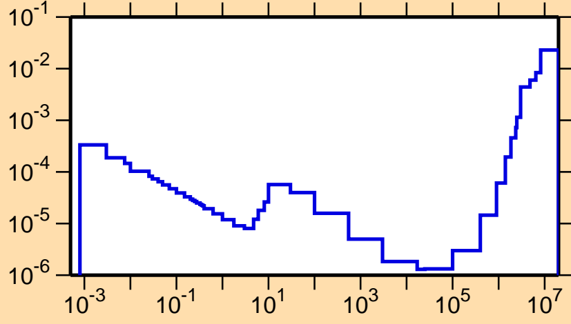
\sigma vs. E for ^{212}\text{Ra}(n,p)
