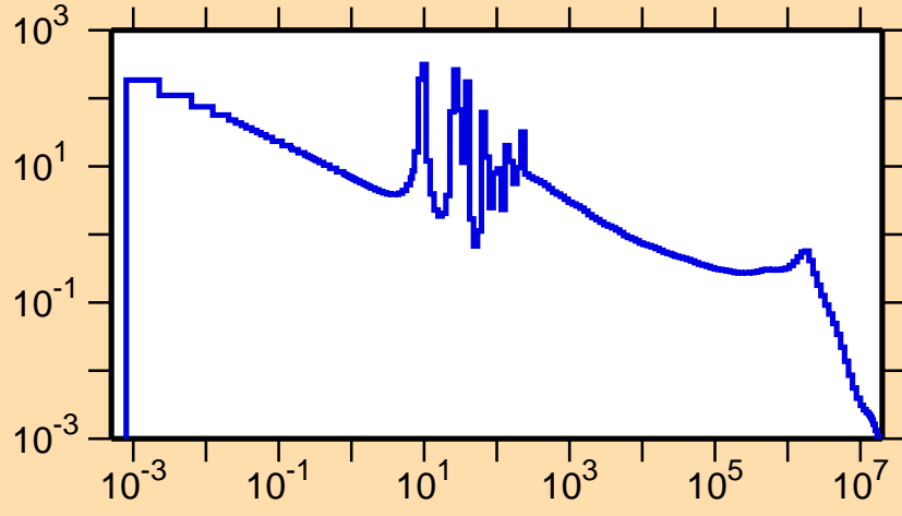
\sigma vs. E for ^{213}\text{Ra}(n,\gamma)
