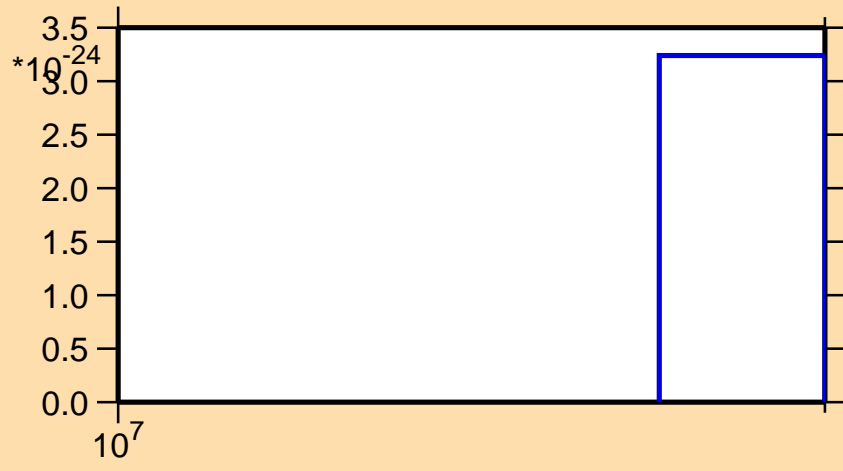
\sigma vs. E for ^{213}\text{Ra} (mt 42)
