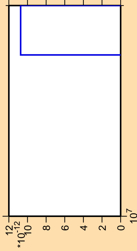
\Delta\sigma/\sigma vs. E for ^{213}\text{Ra} (mt 42)
