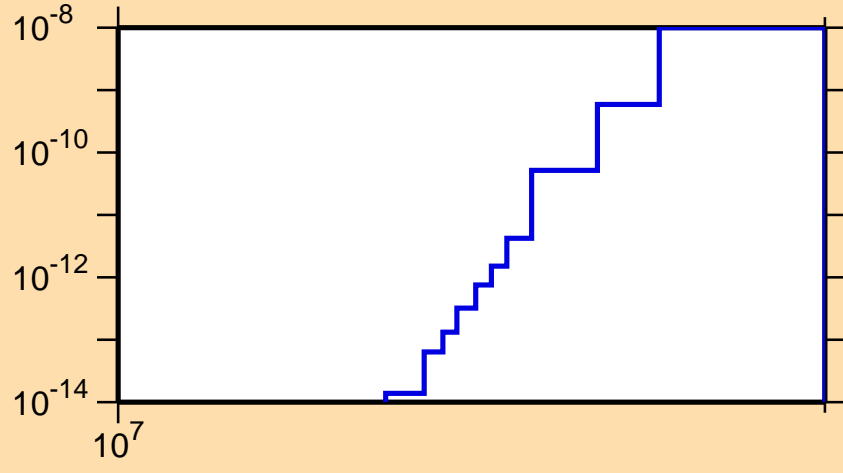
\sigma vs. E for ^{213}\text{Ra}(n,\text{pt})
