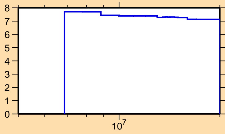
\Delta\sigma/\sigma vs. E for ^{213}\text{Ra}(n,\text{nonel.})
