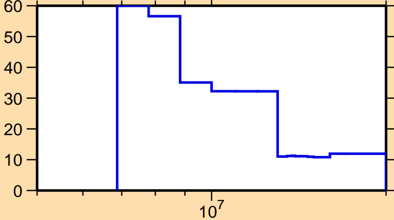
\Delta\sigma/\sigma vs. E for ^{213}\text{Ra}(n,2n)
