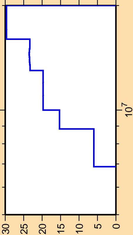
\Delta\sigma/\sigma vs. E for ^{213}\text{Ra}(n,n\text{cont.})
