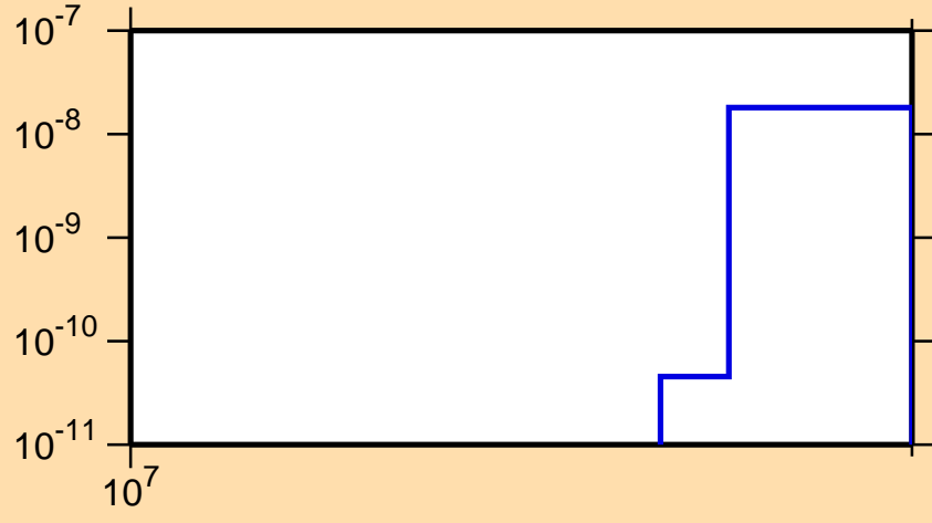
\sigma vs. E for ^{213}\text{Ra}(n,nt)
