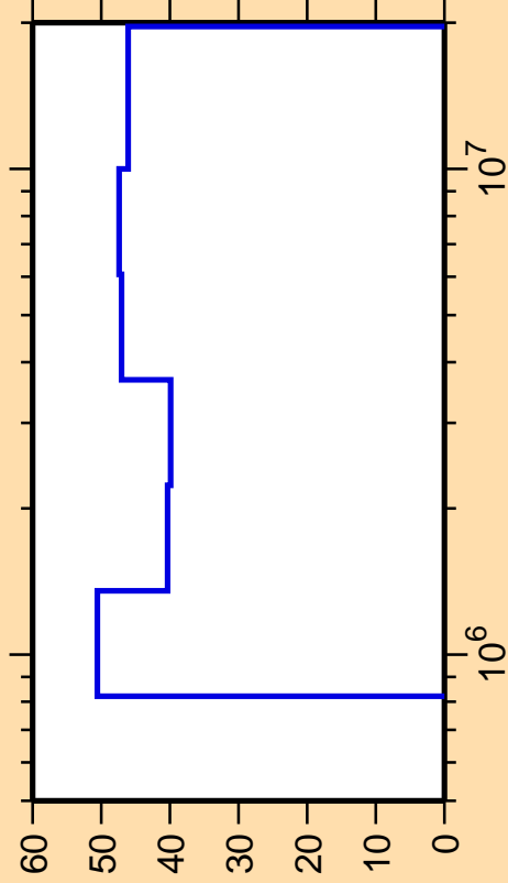
\Delta\sigma/\sigma vs. E for ^{213}\text{Ra}(n,n_2)
