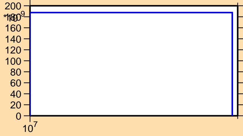
\sigma vs. E for ^{213}\text{Ra}(n,\text{nd})
