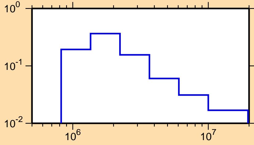
\sigma vs. E for ^{213}\text{Ra}(n,n_2)
