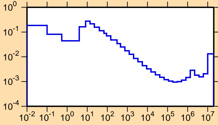
\sigma vs. E for ^{213}\text{Ra}(n,\alpha)
