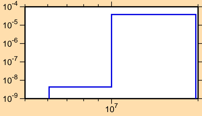
\sigma vs. E for ^{213}\text{Ra}(\text{mt } 45)
